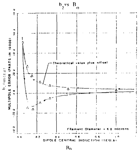
Fig. 1 Normal Sextupole Term
