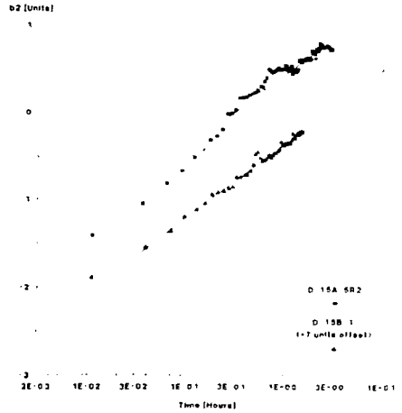
Fig. 4 Sextupole Decay - Two Magnets, Flux Creep Only
