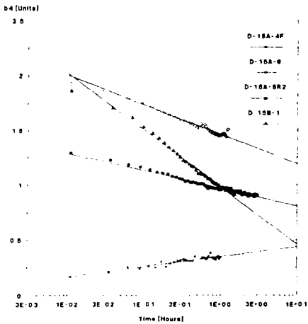
Fig. 3 Decapole Decay - Four Magnets
