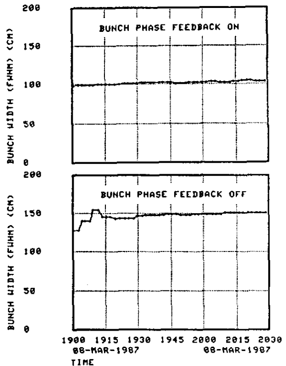
FIGURE 2 Bunch Length Growth with and without Bunch Phase Feedback
