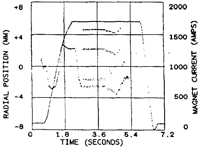
FIGURE 1 Main Ring Ramp and Radial Position. The cogging sequence begins at 2.4 seconds.
