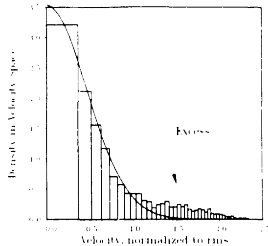
Fig 3 Example of velocity distribution after instability Bicylinder beam \sigma_0 = 90^\circ, \sigma = 41^\circ
