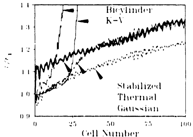
Fig. 1 Comparison of emittance growth of beams with various initial distributions: \sigma_0 = 90^\circ , \sigma_1 = 41^\circ . The bicylinder beam saturates at \epsilon/\epsilon_0 = 2.1 , the K-V beam at \epsilon/\epsilon_0 = 2.5 .
