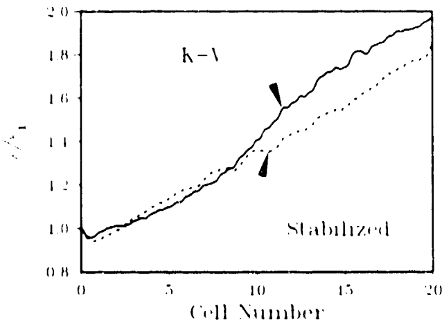
Fig 6 Comparison of beam emittance growth with \sigma_0 = 90^\circ, \sigma = 9^\circ
