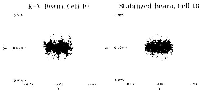
Fig 5 The K-V and stabilized beams \sigma_0 = 90^\circ, \sigma = 9^\circ .
