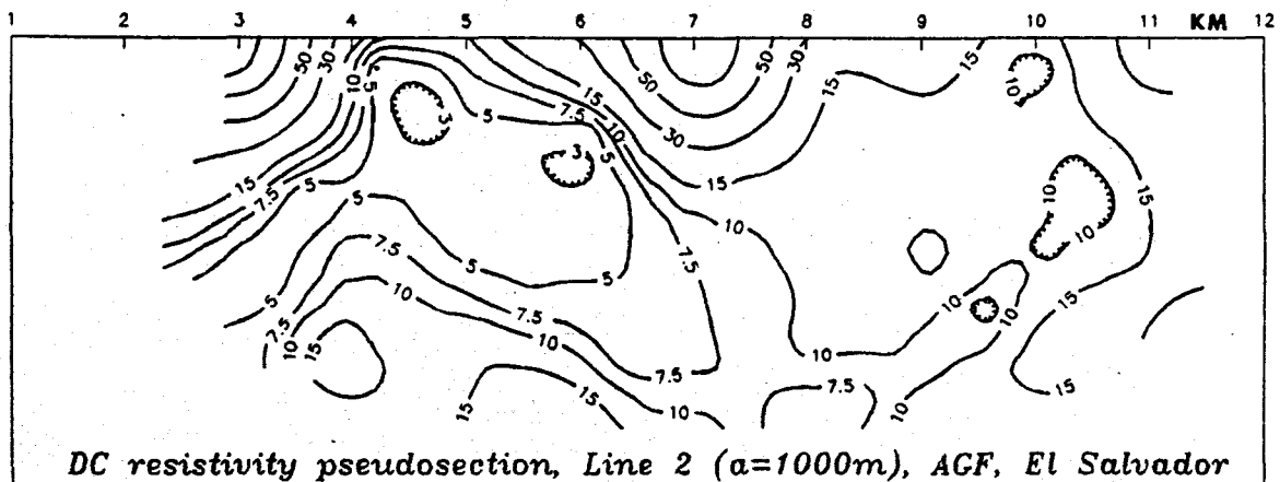
Fig. 7. Pseudosection of Line 2 showing the apparent resistivities logarithmically contoured in ohm-meters for 1000 meter dipole spacing.
