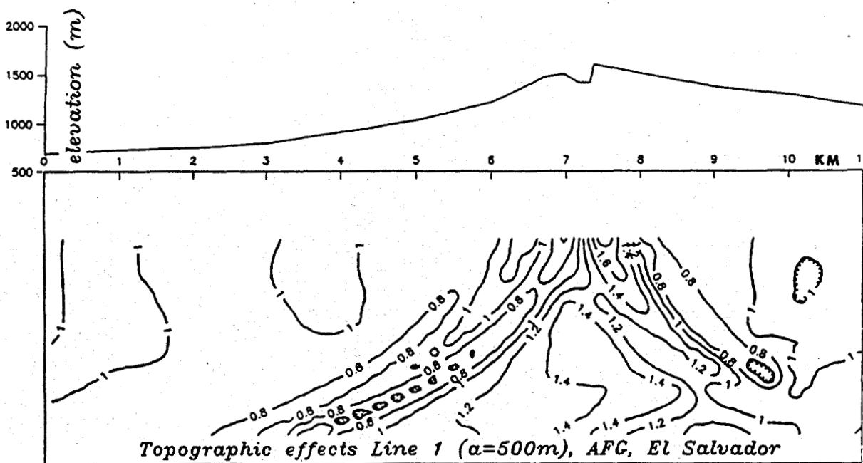
Fig. 6. Logarithmic pseudosection of topographic effects on Line 1 due to the mountains south of the site for 500 meter dipole spacings.
