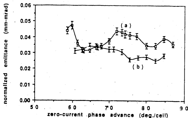
Fig. 3. Emittance measurements at l.p. 20 for coherent amplitudes of (a) 4.5 mm and (b) 1.9 mm.
