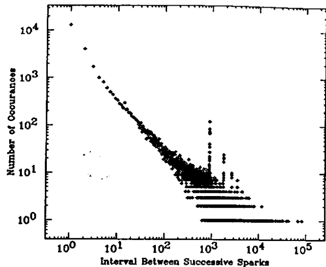
Fig. 4. Histogram of the interval between successive sparks.
