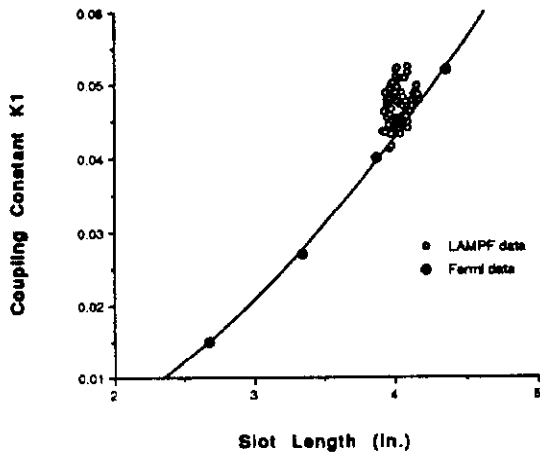
Figure 2: SCC Slot Length vs Nearest Neighbor Coupling Constant, k_1
