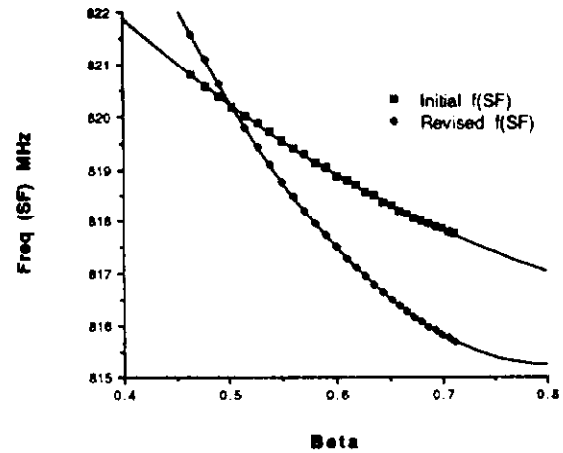
Figure 4: f_{SF} vs \beta for the Fermilab SCC
