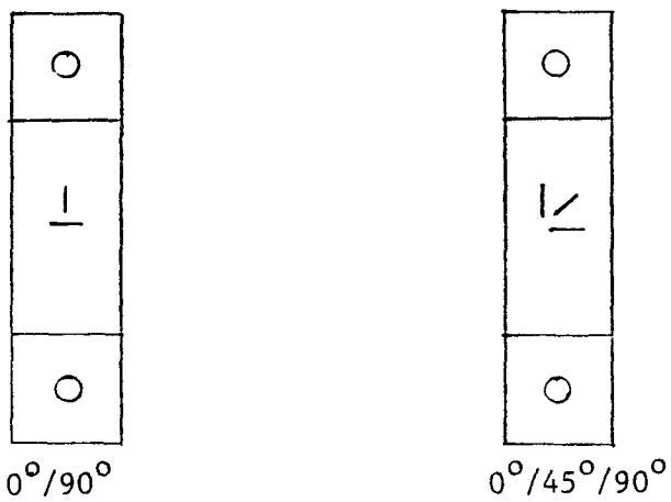
Fig. 2: Strain gauge configurations for test coupons
