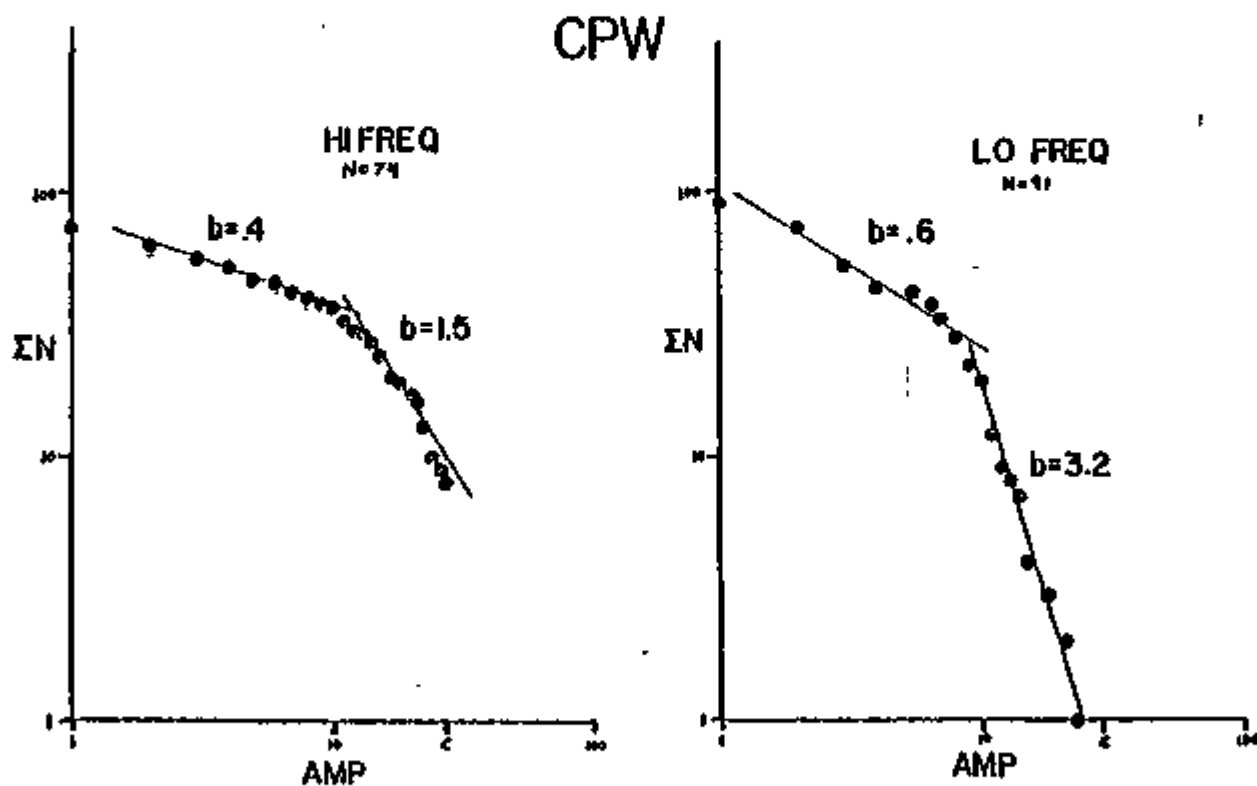
Figure 16. B-value plots for May 14 - May 18 volcanic earthquakes from Mt. St. Helens. Both high frequency (left) and low frequency (right) events show a break in slope, again indicating that two physical mechanisms are acting.
