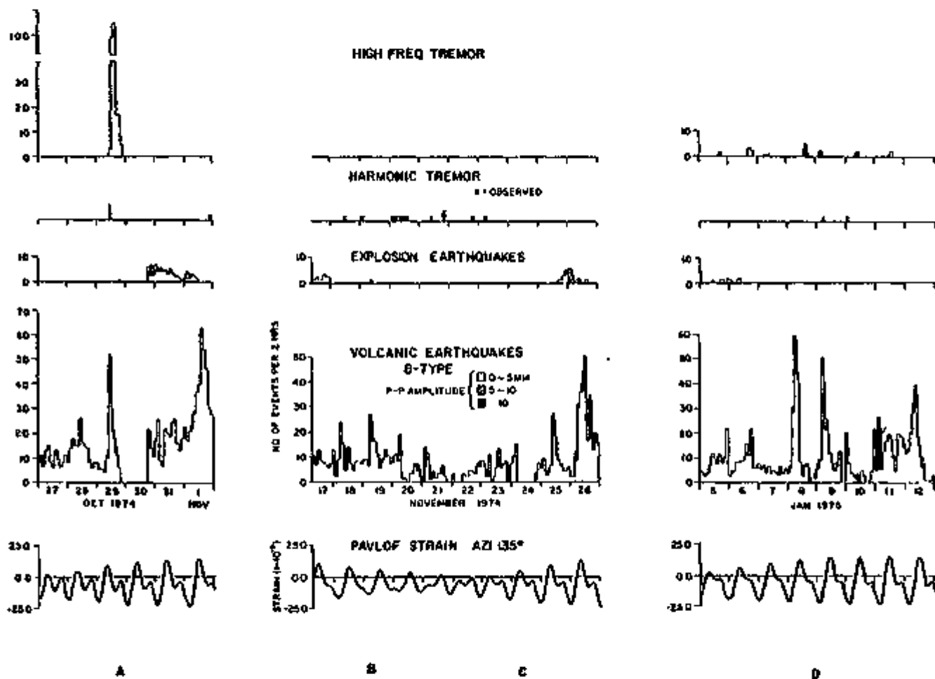
Figure 12. Comparison of different types of Pavlof volcano seismicity with horizontal tidal strain across the Aleutian arc. Note in particular the relation between the traces for the number of volcanic B-type earthquakes and the solid earth tidal strain in azimuth 135°. A and C label the beginning of eruptions, while B and D label the ends of eruptions. Note that during A and C peaks in the number of earthquakes just follow positive peaks in strain, while during B and D they just follow negative peaks in strain. It appears possible to interpret these data in terms of inflation and deflation, respectively, at the volcano prior to and following an eruption. Note that in this particular case ocean-load stresses were not accounted for and only astronomical solid-earth tides were computed.
