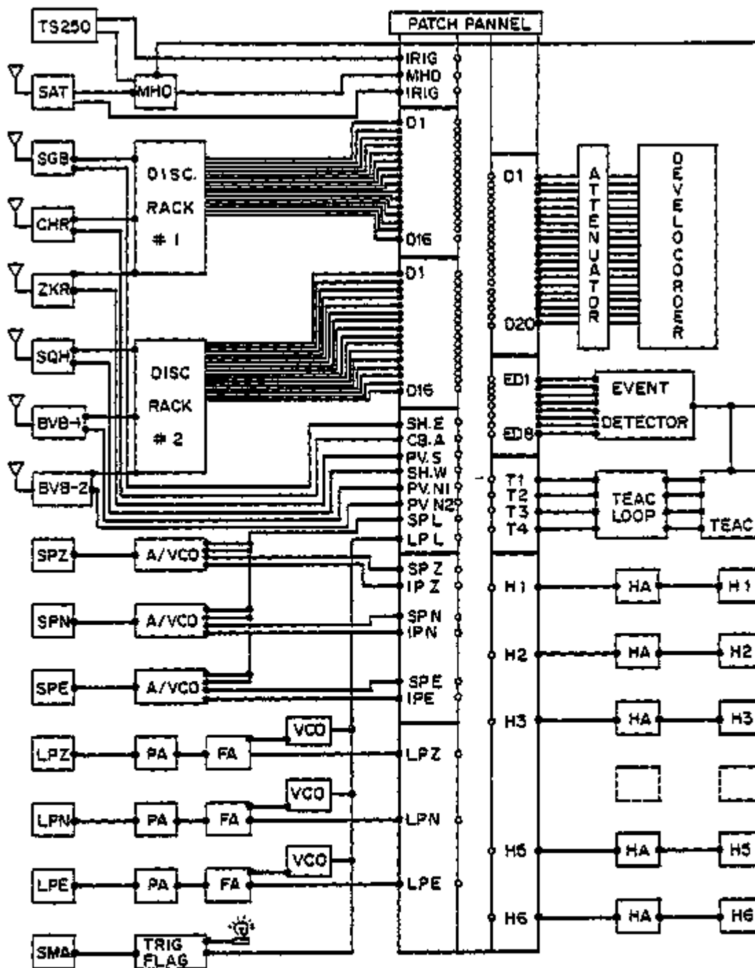
Figure 29. Block diagram for the Sand Point recording center, September 1980. Signal sources are arrayed down the far left of the diagram, signal conditioners are in the middle left, the patch panel in the center, and the recording devices on the right. Signal sources: Sprengnether TS250 chronometer; Kinemetrics satellite receiver for CDT; VHF receivers for subnetworks of the remote seismic stations - SGB (Shumagin-east subnet, SH.E), CHR (Cold Bay subnet, CB.A), ZKR (Pavlof-south subnet, PV.S), SQH (Shumagin-west subnet, SH.W), BVB-1 (Pavlof-north-1 subnet, PV.N1) and BVB-2 (Pavlof-north-2 subnet, PV.N2); SPZ, N and E, the local Baby Benioff, short-period seismometers; LPZ the local Sprengnether long-period vertical seismometer; LPN and E, the local Geotech long-period, horizontal seismometers; and Kinemetrics SMA-1 (1G) strong-motion accelerometer. Signal conditioners: L-DGO min.-hr.-day (MHO) board; discriminator racks 1 and 2; L-DGO two-channel amplifier-VCO units (A-VCO); L-DGO pre- and filter amplifiers (PA and FA) and modified Emel 6202 VCO, for the long-period signals; and the L-DGO trigger-flag board. All of the signals are available on the patch panel where they can be routed to the event-detector and/or any recording device: Developcorder (18 data channels plus two for time); TEAC tape recorder (four channels, 32 seismic tones plus IRIG time code and tape-speed compensations tones); 5 Helicorders (one channel each, HA = Helicorder amplifier). Note that only the multiplexed output (SH.E through LP.L) are input to the TEAC system and that this system only records when the event-detector declares an event (see Figure 28).
