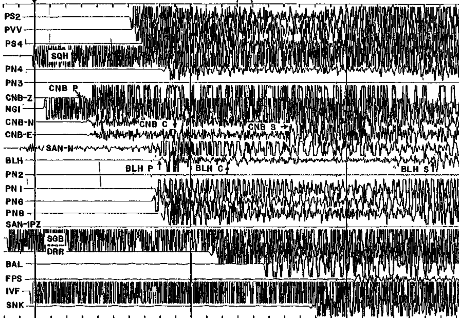
Figure 30b. Sample Versatec record from 15:36 day 221, 1980. This record was created by digitizing the demodulated TEAC tape and then plotting the digital data on a versatec plotter using the PDP 11/70. Note that many of the traces are unclipped and the whole waveform is available for analysis; for examples, note that the signals from CNB and BLH show clear P-, S- and converted (C) phases; these are labelled CNB P, CNB S, CNB C, BLH P, BLH S, and BLH C, respectively.
