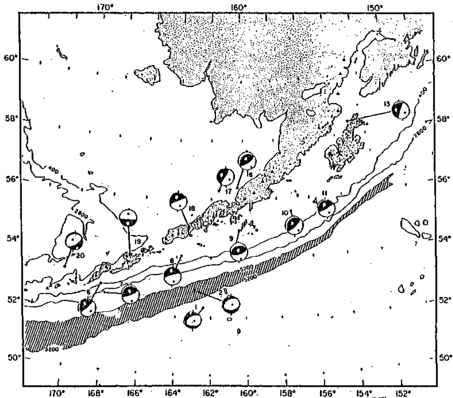
Figure 17. Focal mechanisms (Davies et al., 1980) of earthquakes analyzed in this study.
