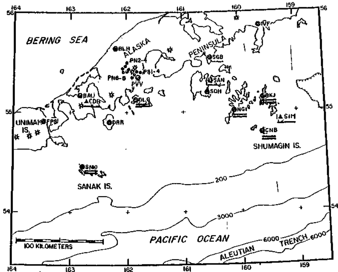
Figure 26. Shumagin Network (see Figure 23 for location). Remote stations with a single, vertical geophone are shown with filled circles. Stations with three orthogonal seismometers (CMB and SAN) are shown with a filled hexagon. Network stations with SMA-1 strong-motion accelerographs (SMK, NCI, DLG, SCB, BKJ, SAN, CMB) are indicated by the heavy line under the designator code. Those with double underlining transmit on SMA trigger signal; when one of these SMA's is triggered, a tone is sent via the VHF telemetry system to a detector at SAN which turns on the tape recorder. The triangles at SIM and CDB indicate SMA-1's unrelated to any network station. The SAN station has three orthogonal long period seismographs as well as the short and intermediate period system similar to that at DUT (see caption from Figure 25). Signals at SAN are recorded on an event detecting magnetic tape recorder, a Develocorder and 5 Helicorders; records from these devices are processed at L-DCO.
