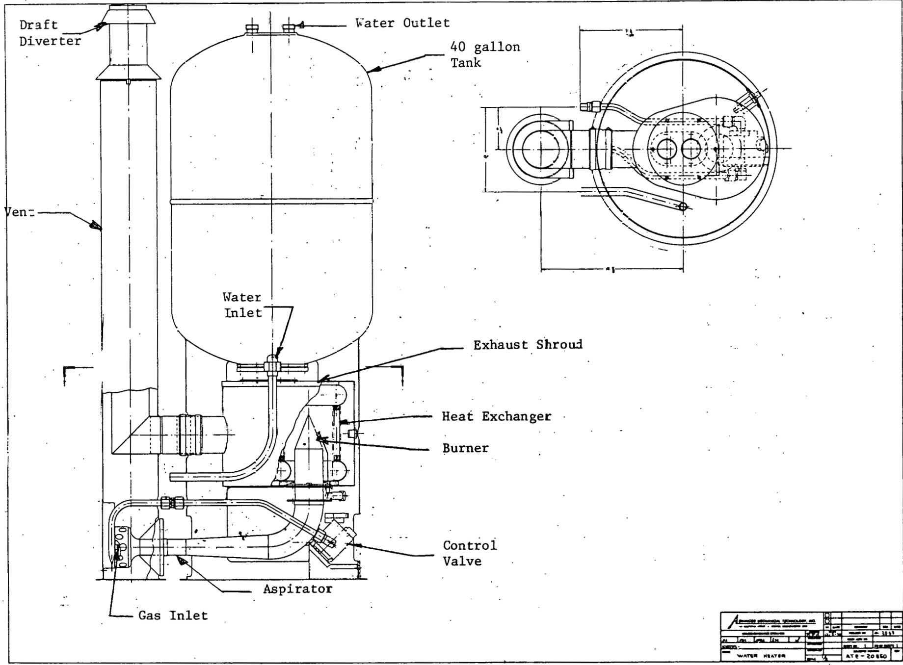
Figure 3. Prototype Water Heater Design
