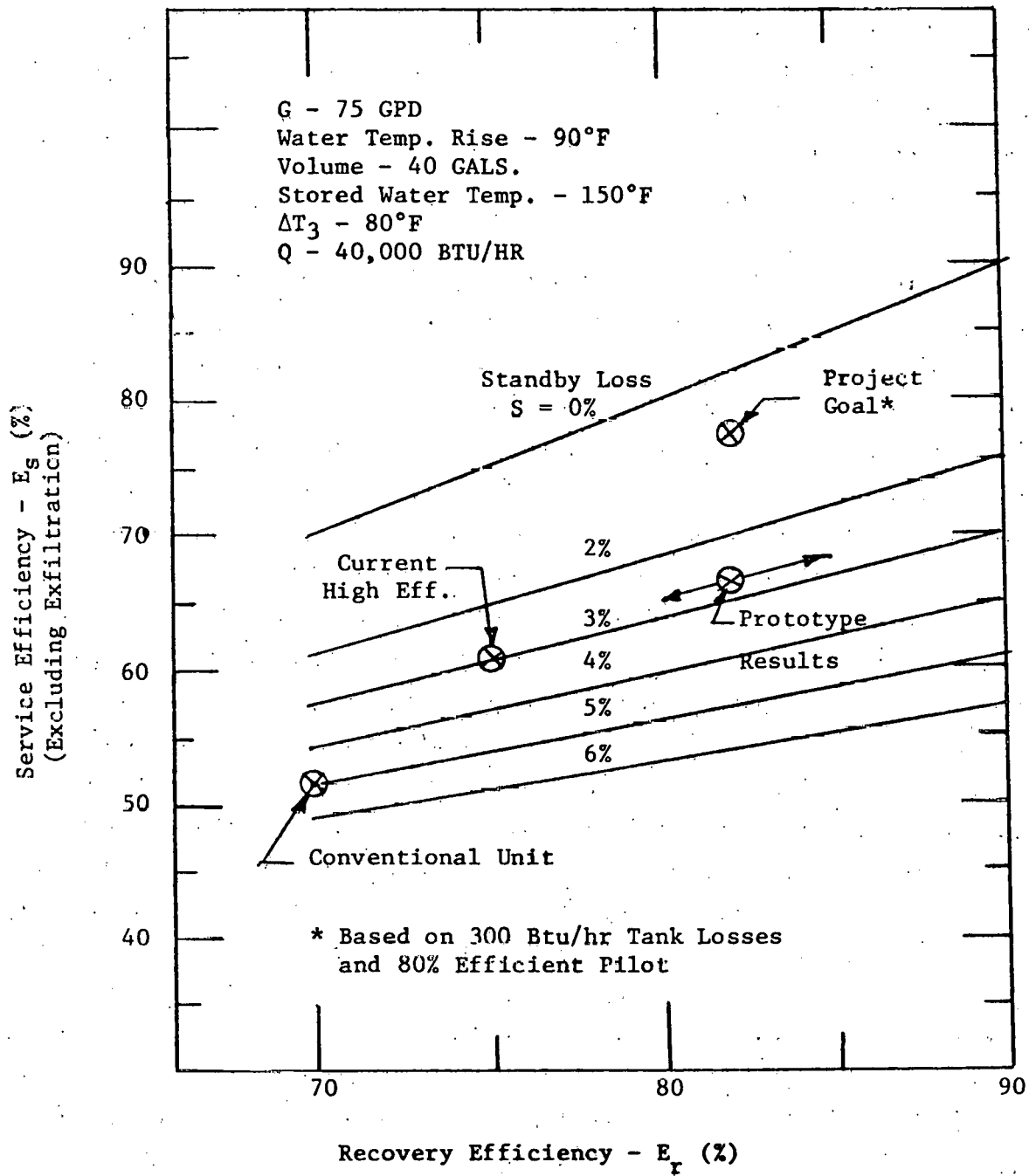
Figure 7. Service Efficiency Versus Recovery Efficiency at Various Standby Losses
