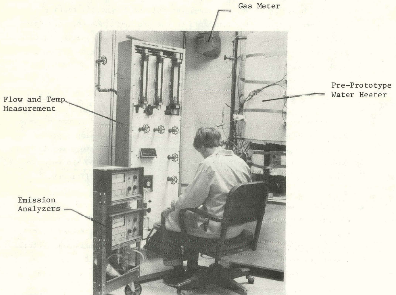
Figure 6. Pre-Prototype Water Heater Installed in Test Facility
