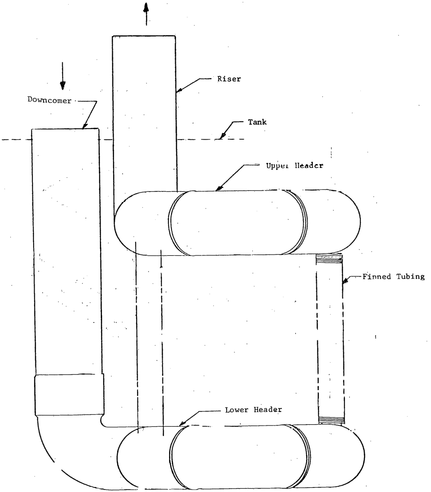
Figure 5. Heat Exchanger Configuration
