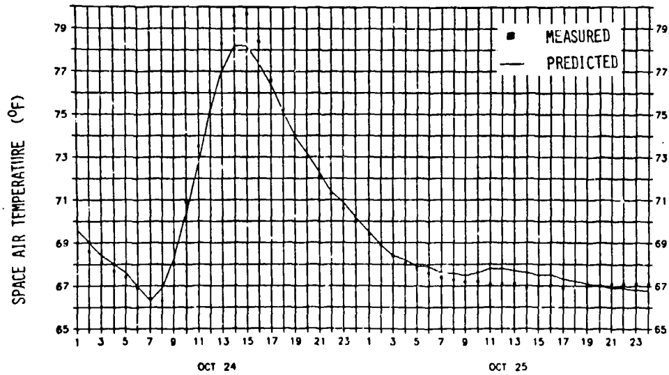
Fig. 2. Measured and predicted space air temperatures for the October 1981 NBS direct-gain test cell data.
