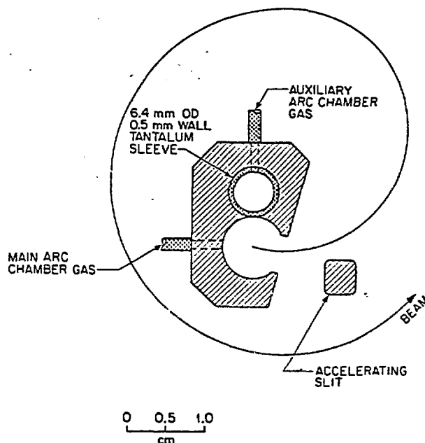
Fig. 1. Median plane cross section of the dual arc chamber source. The arcs in the two chambers share a single cathode at each end.
