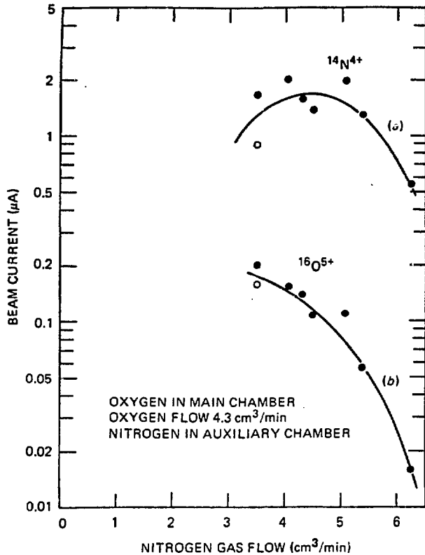
Fig. 6. Curve 6(a) is the intensity of ^{14}\text{N}^{4+} beam with nitrogen admitted to the auxiliary chamber. Curve 6(b) is the ^{16}\text{O}^{5+} beam intensity with oxygen admitted to the main chamber.
