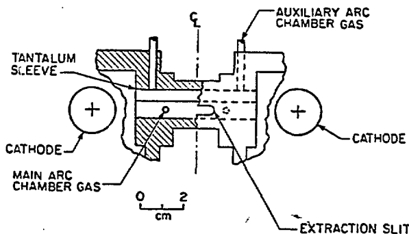
Fig. 2. Front view of the dual arc chamber source with a section removed to show the gas entry port to the main arc chamber and the cathode position in relation to the main and auxiliary arc chambers.
