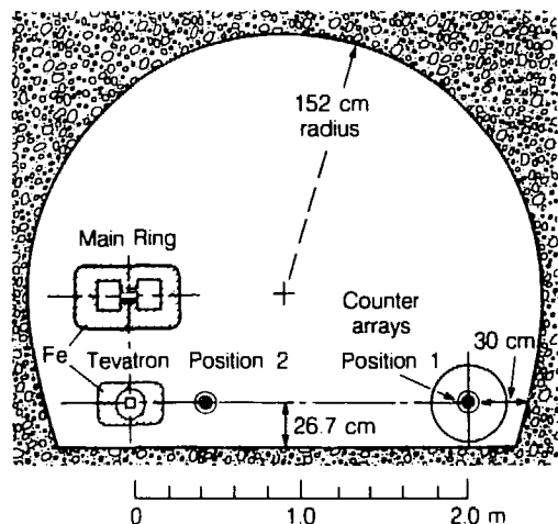
Fig. 2. Tunnel cross section near A-17.
