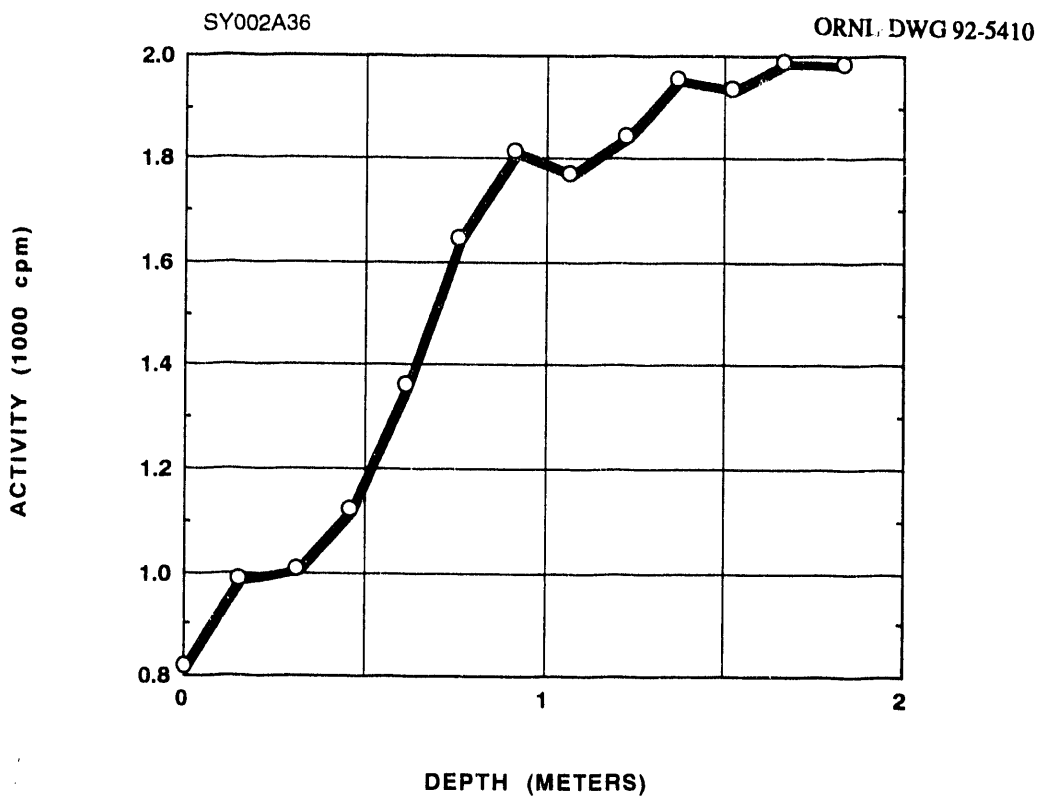
Fig. A.35. Gamma profile of auger hole A036.
