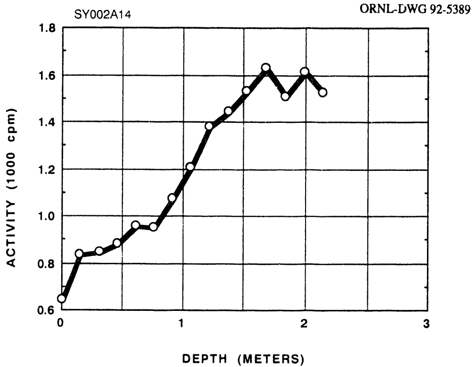
Fig. A.14. Gamma profile of auger hole A014.
