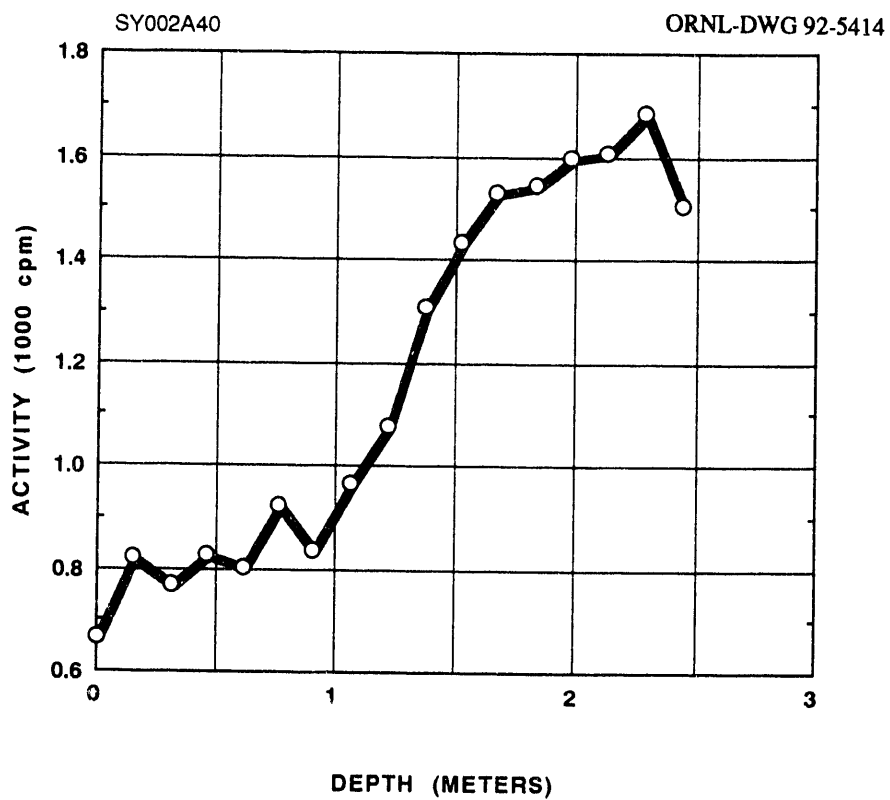
Fig. A.39. Gamma profile of auger hole A040.
