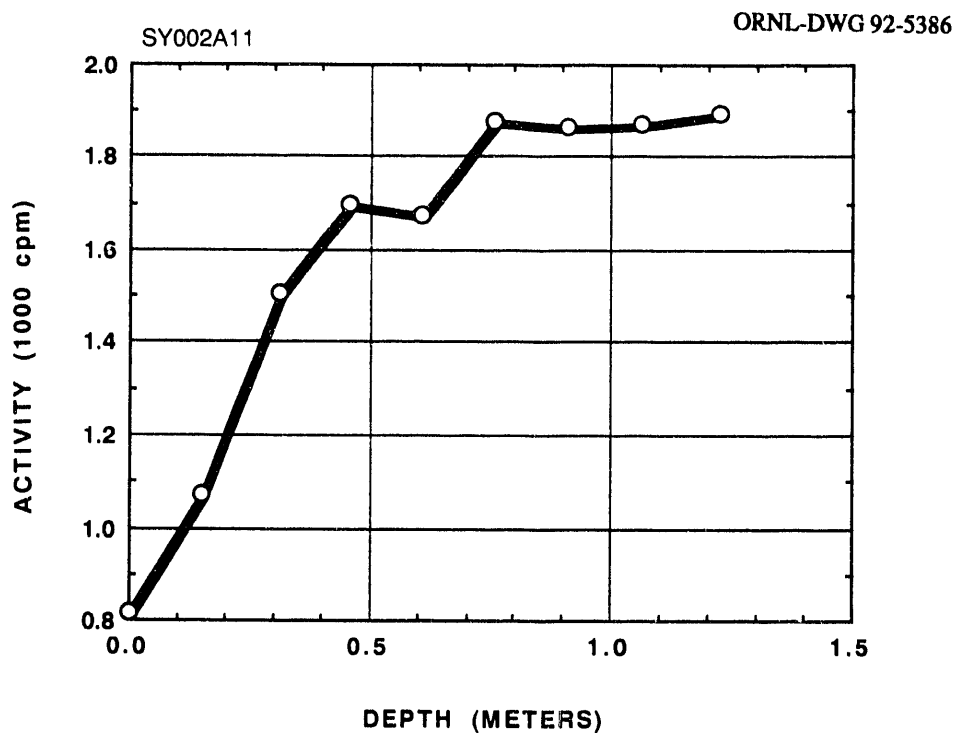
Fig. A.11. Gamma profile of auger hole A011.
