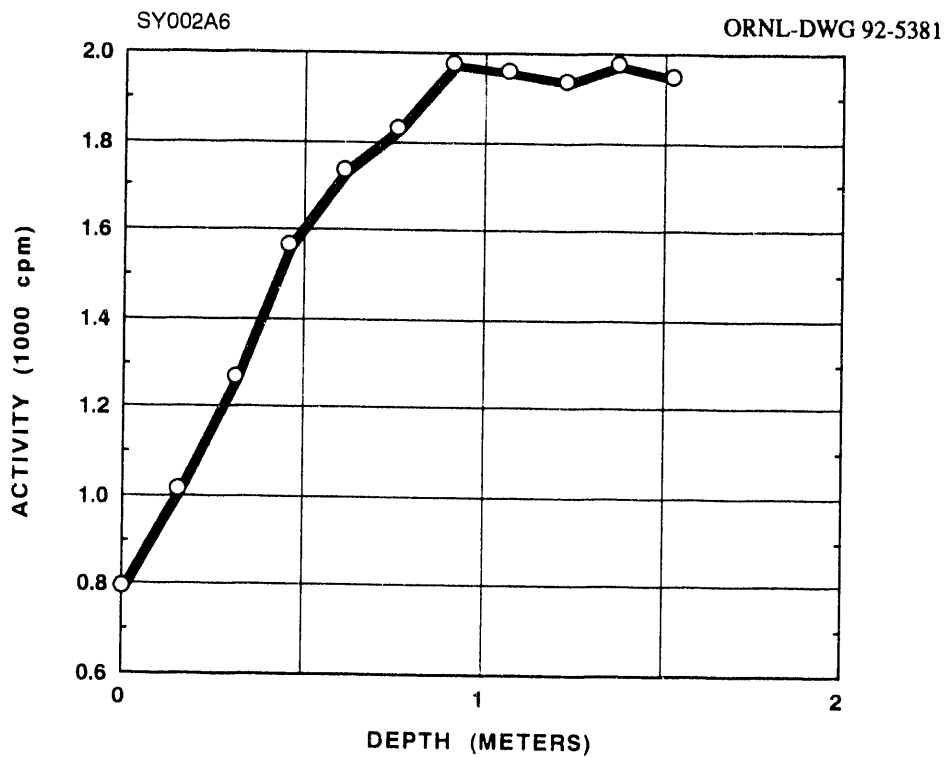
Fig. A.6. Gamma profile of auger hole A006.
