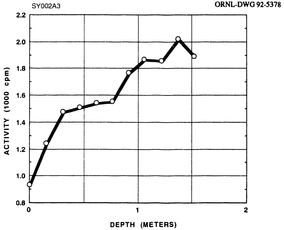
Fig. A.3. Gamma profile of auger hole A003.
