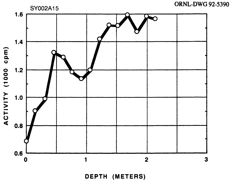
Fig. A.15. Gamma profile of auger hole A015.
