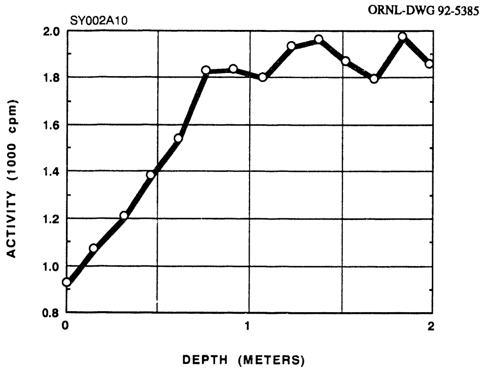
Fig. A.10. Gamma profile of auger hole A010.
