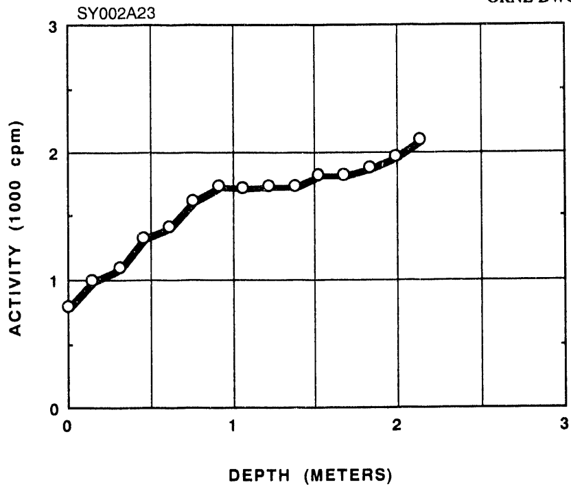
Fig. A.23. Gamma profile of auger hole A023.
