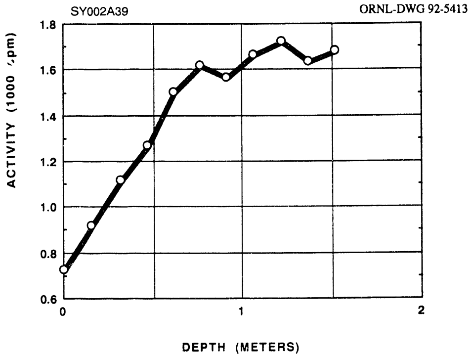
Fig. A.38. Gamma profile of auger hole A039.
