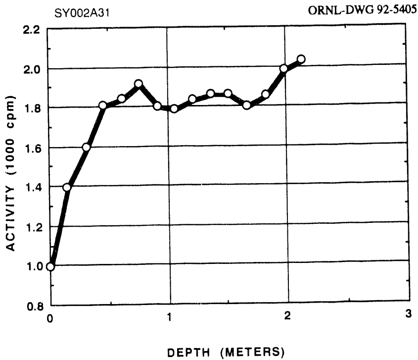
Fig. A.30. Gamma profile of auger hole A031.
