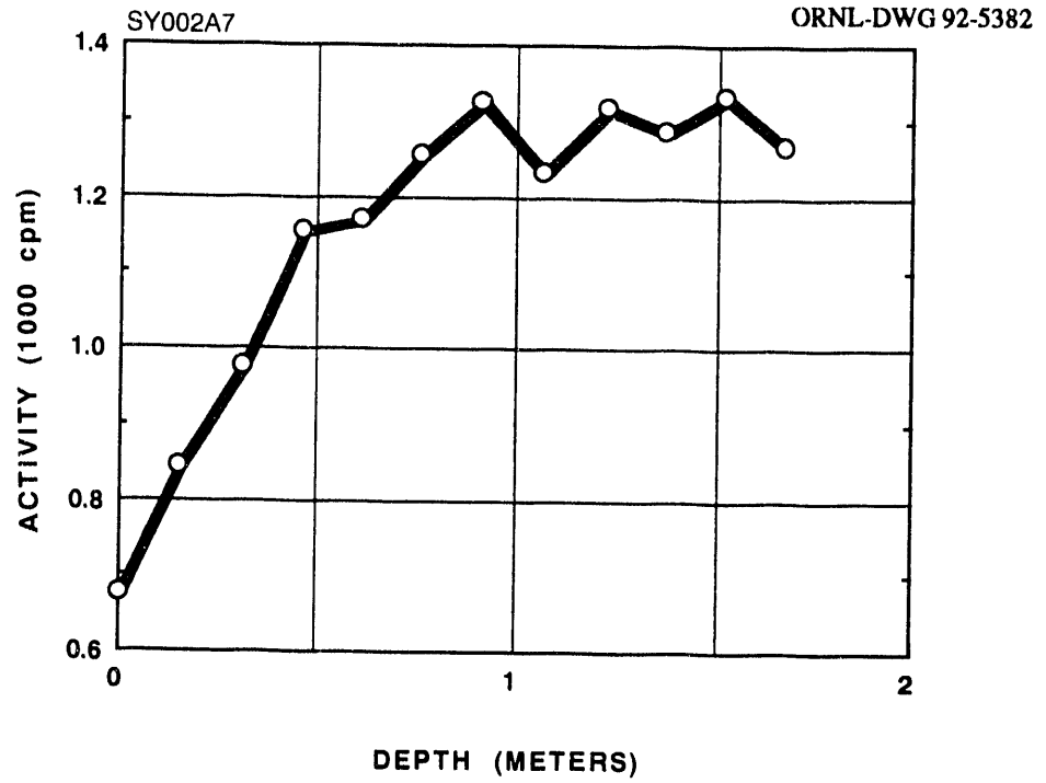
Fig. A.7. Gamma profile of auger hole A007.
