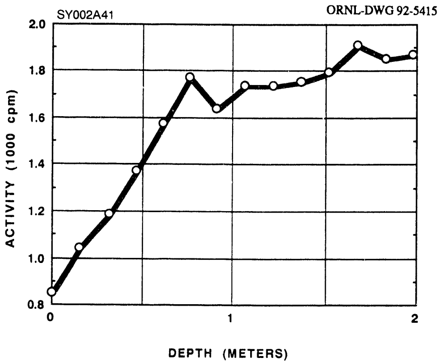
Fig. A.40. Gamma profile of auger hole A041.
