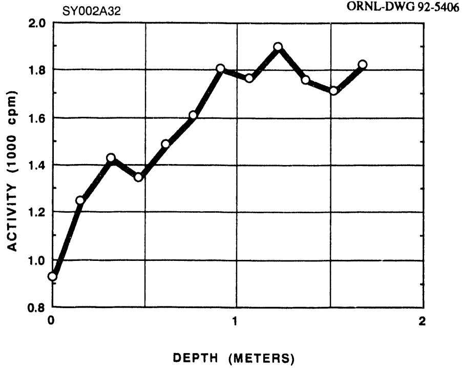
Fig. A.31. Gamma profile of auger hole A032.
