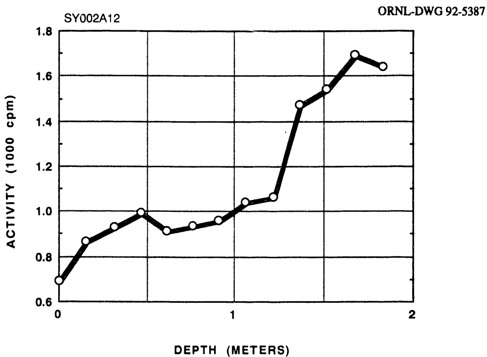
Fig. A.12. Gamma profile of auger hole A012.
