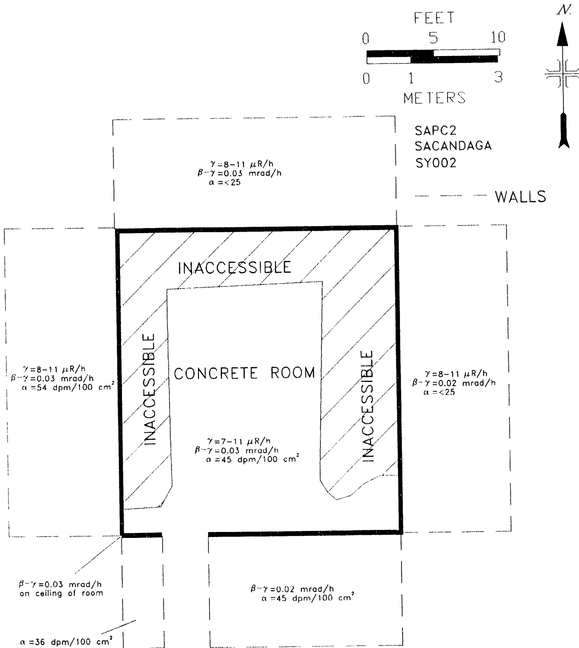
Fig. 14. Directly measured radiation levels inside the concrete room, building P at the Sacandaga site.
