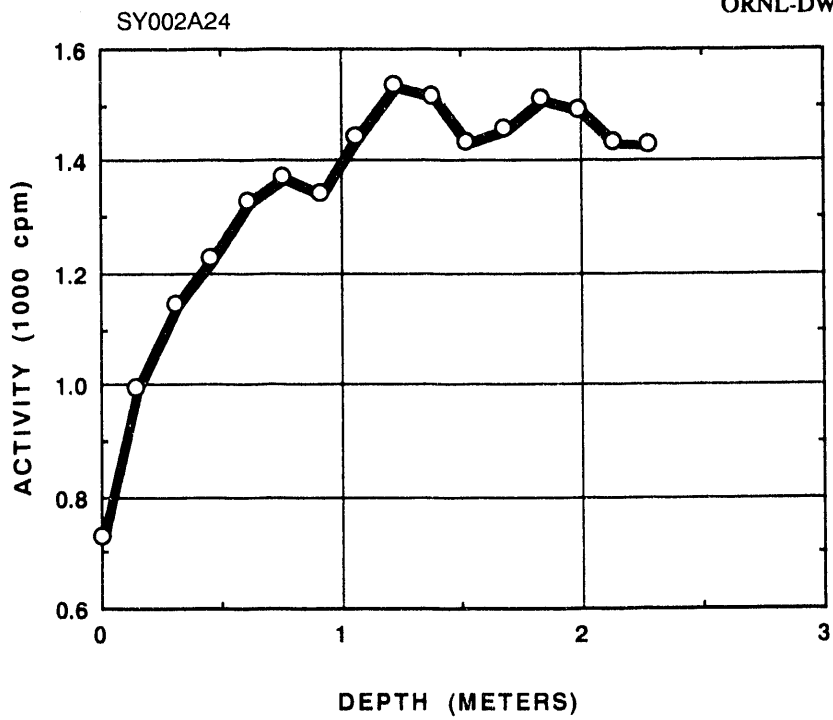
Fig. A.24. Gamma profile of auger hole A024.
