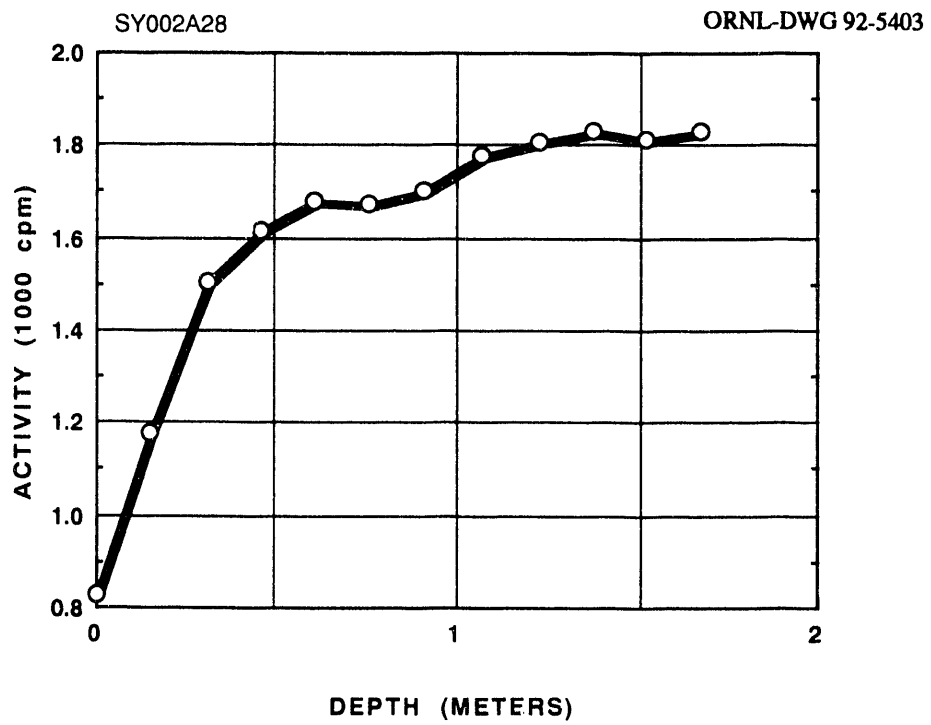
Fig. A.28. Gamma profile of auger hole A028.
