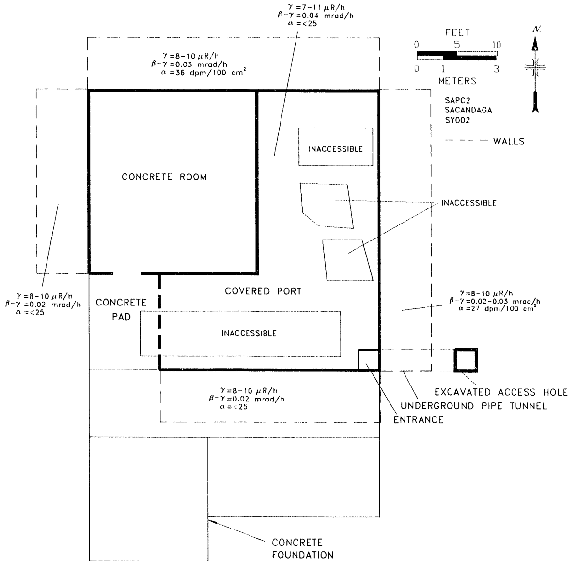
Fig. 13. Directly measured radiation levels inside the covered port of building P at the Sacandaga site.
