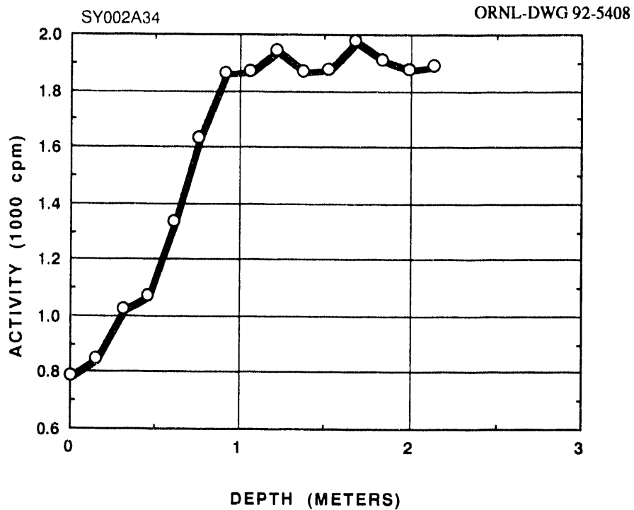
Fig. A.33. Gamma profile of auger hole A034.
