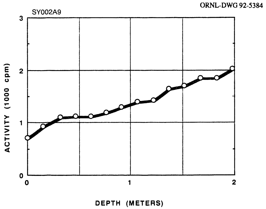
Fig. A.9. Gamma profile of auger hole A009.
