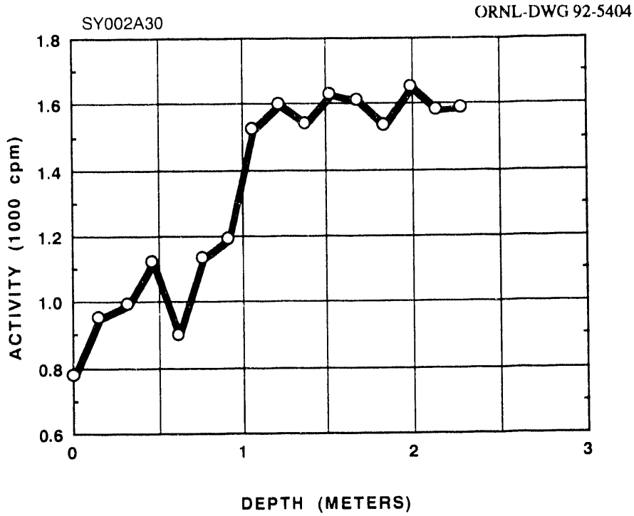
Fig. A.29. Gamma profile of auger hole A030.
