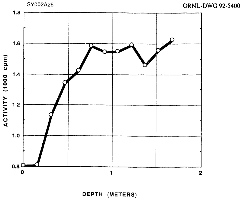
Fig. A.25. Gamma profile of auger hole A025.
