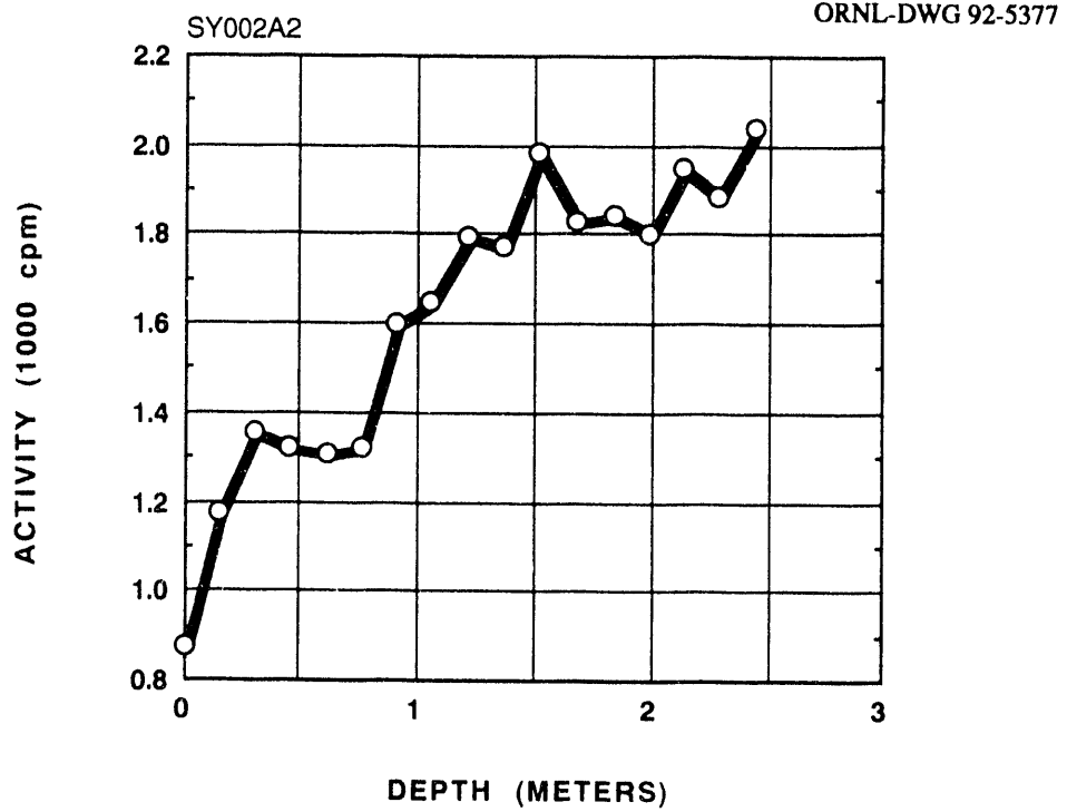
Fig. A.2. Gamma profile of auger hole A002.
