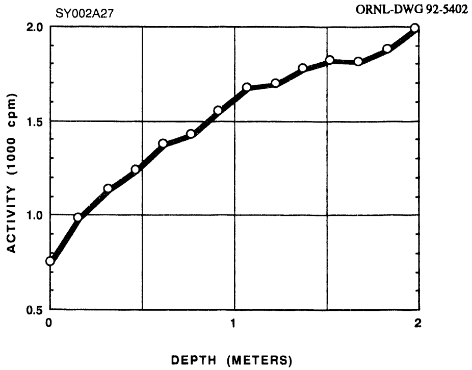
Fig. A.27. Gamma profile of auger hole A027.
