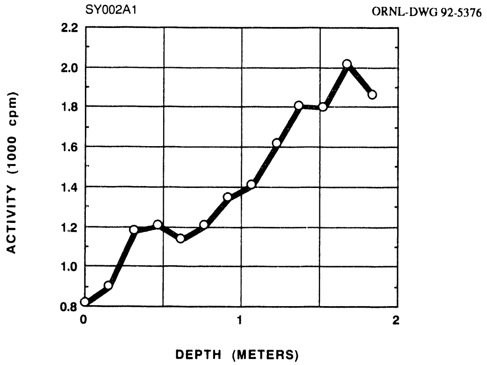
Fig. A.1. Gamma profile of auger hole A001.
