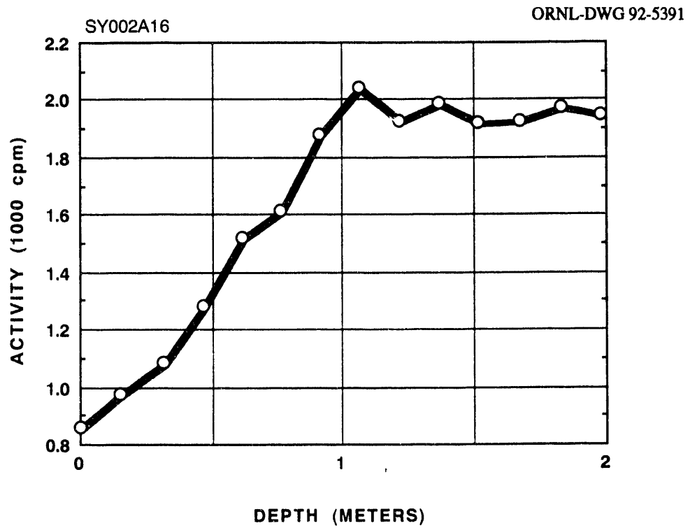
Fig. A.16. Gamma profile of auger hole A016.
