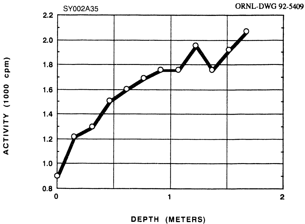
Fig. A.34. Gamma profile of auger hole A035.
