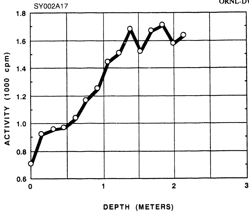
Fig. A.17. Gamma profile of auger hole A017.
