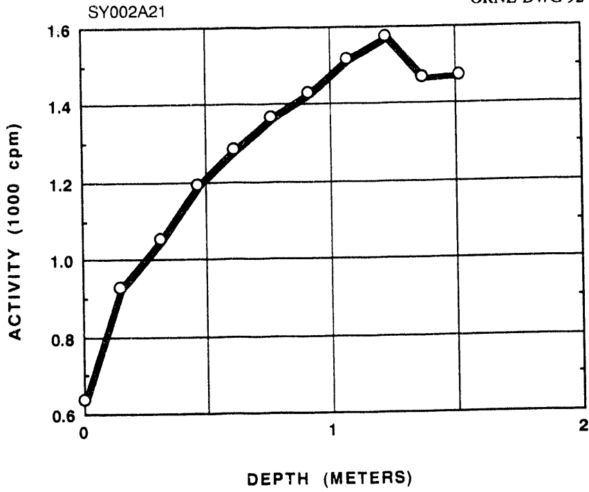
Fig. A.21. Gamma profile of auger hole A021.
