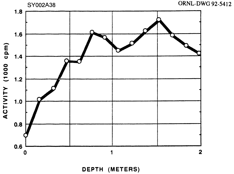
Fig. A.37. Gamma profile of auger hole A038.
