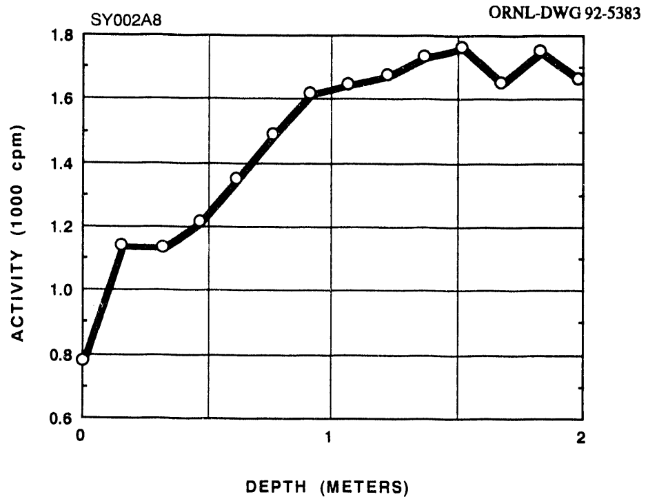
Fig. A.8. Gamma profile of auger hole A008.
