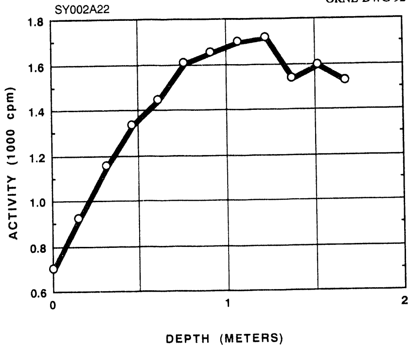
Fig. A.22. Gamma profile of auger hole A022.
