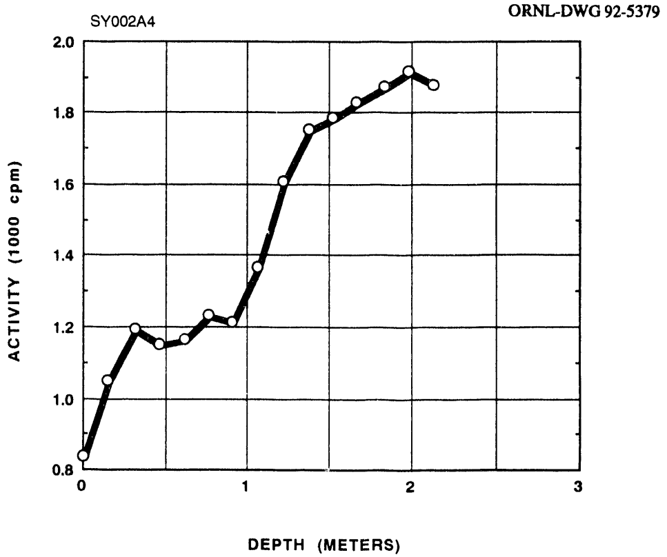
Fig. A.4. Gamma profile of auger hole A004.
