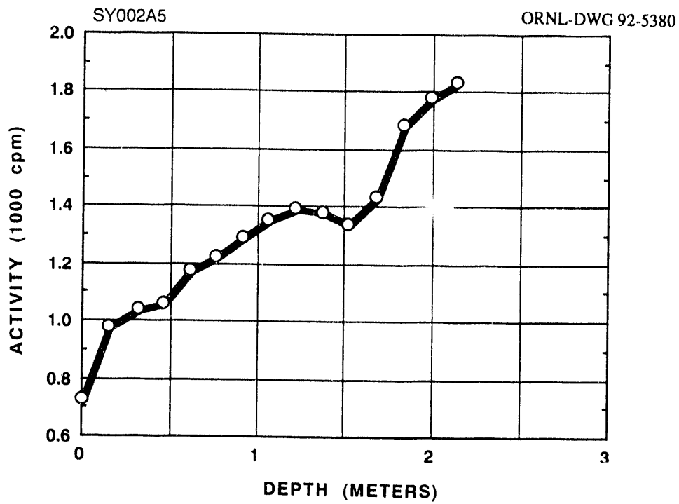
Fig. A.5. Gamma profile of auger hole A005.
