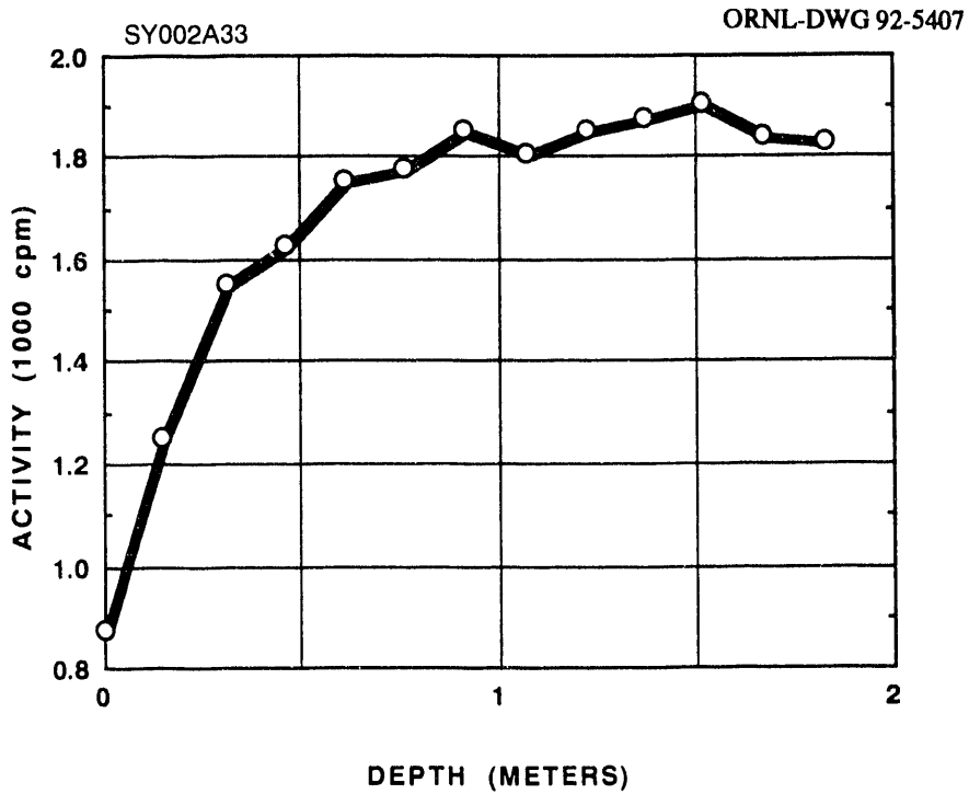
Fig. A.32. Gamma profile of auger hole A033.
