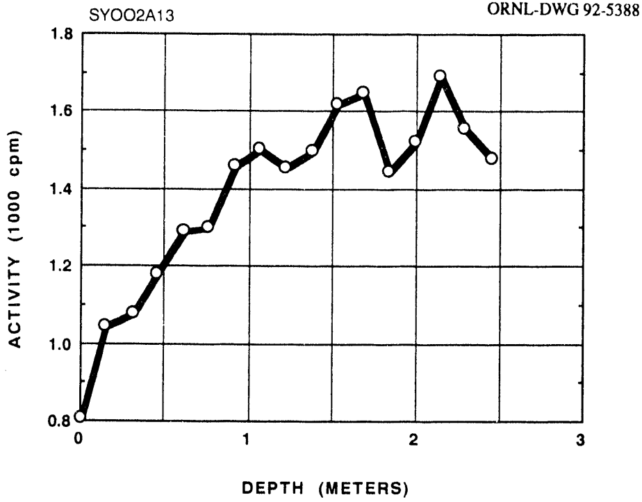
Fig. A.13. Gamma profile of auger hole A013.
