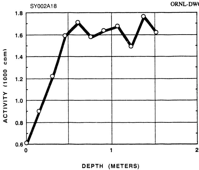
Fig. A.18. Gamma profile of auger hole A018.
