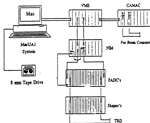
DAQ SYSTEM FOR TRD BEAM TEST
