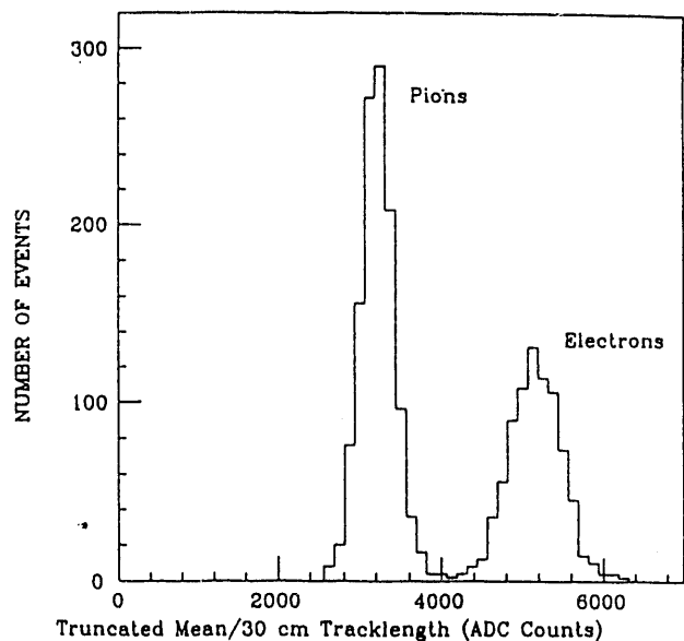
Figure 7: Electron, pion dE/dx distribution for 30 cm track length and 60% truncated mean. The data is for particles with momenta 1.0 GeV/c and 35^\circ incident angle.
