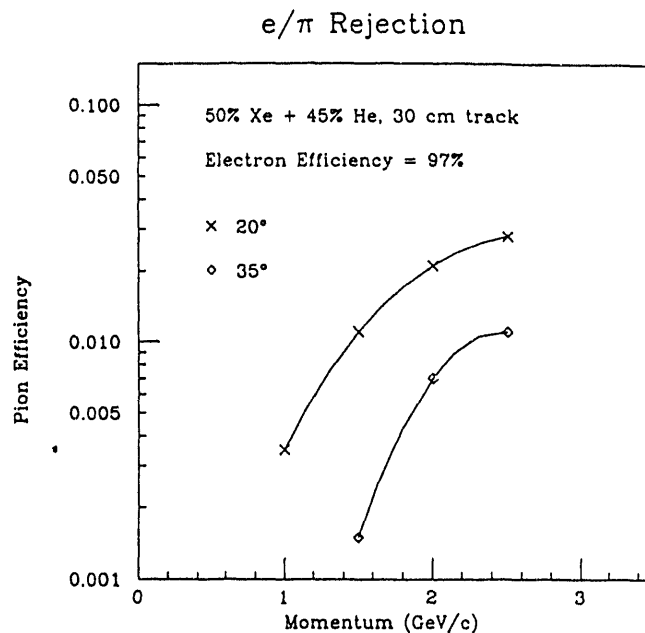
Figure 9: dE/dx e/\pi rejection for 97% electron efficiency and 50% Xe + 45% He + 5% C_4H_{10} gas. The track length is 30 cm and the incident angles are 20^\circ and 35^\circ .
