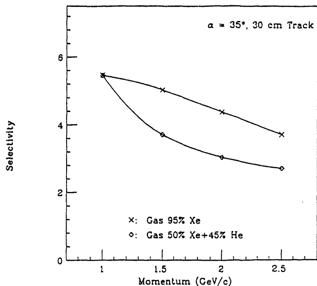
Figure 8: S-value for 2 different gas mixtures. 95% Xe + 5% C_4H_{10} and 50% Xe + 45% He + 5% C_4H_{10} . The data is for 30 cm track length and 35^\circ incident angle.
