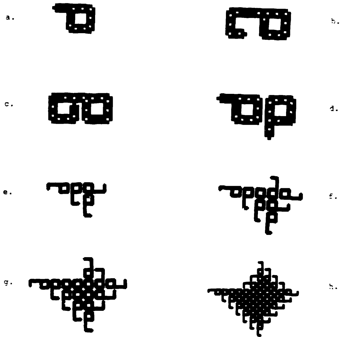
Figure 2: A cellular automaton model of self-replication, due to Chris Langton. Signals propagating around the "Adam" loop (a) cause the short arm to grow and curl back on itself (b,c,d), producing an offspring loop (e). Each loop then goes on to produce further offspring, which also reproduce (f). This process continues indefinitely, resulting in an expanding colony of loops (g,h), consisting of a "living" reproductive fringe surrounding a growing "dead" core, as in the growth of a coral.
