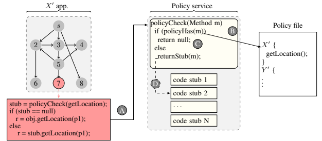
Figure 4: Step 3: Enforcing the Policy
