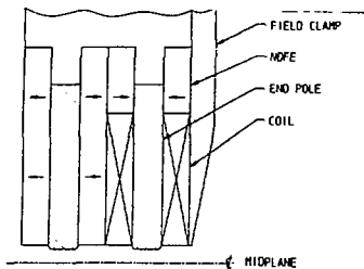
Figure 2. End Pole Configuration
