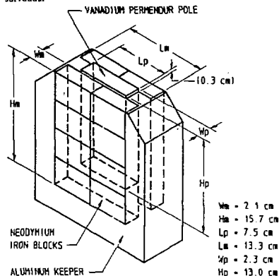
Figure 1. Half Period Pole Assembly
