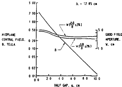
Figure 3. Prototype Pole Magnetic Measurements
