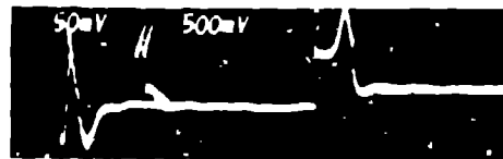
Fig. 5. Cavity phase error 50 mV/deg. (50 mV, 200 \mu s/div).
