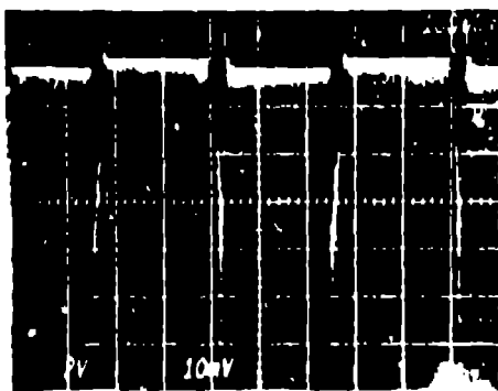
Fig. 4. Vertically expanded cavity field with simulated 200% beam loading. Full signal is 240 mV P-P. (10 mV, 100 \mu s/div).
