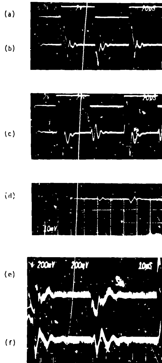
Fig. 3. (a) External demand on slave controller (2 V, 20 ns/div). (b) Slave amplitude error signal (100 mV, 20 ns/div). (c) Cavity amplitude error signal (100 mV, 20 ns/div). (d) Cavity rf field (10 mV, 20 ns/div). (e) Vertically expanded envelope of master chain. Full envelope is 2V P-P. (200 mV, 10 ns/div). (f) Vertically expanded rf envelope of slave chain. Full envelope is 2V P-P. (200 mV, 10 ns/div).
