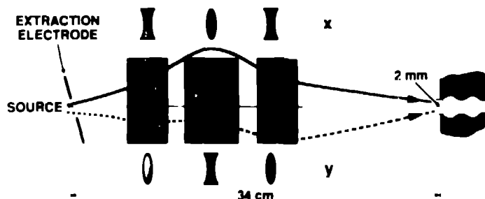
Fig. 1. Schematic of the LEBT transport from the source to the RFQ
