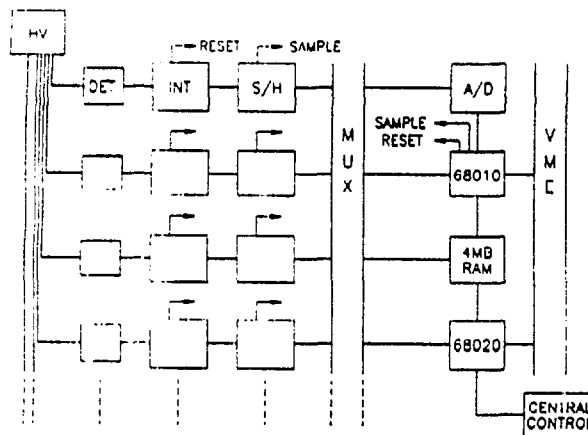
Fig. 5 Block Diagram of Upgraded System.
