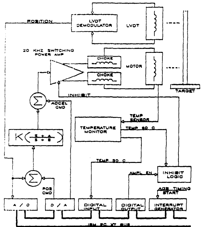
Figure 2. Block diagram of the beam scaper control system.
