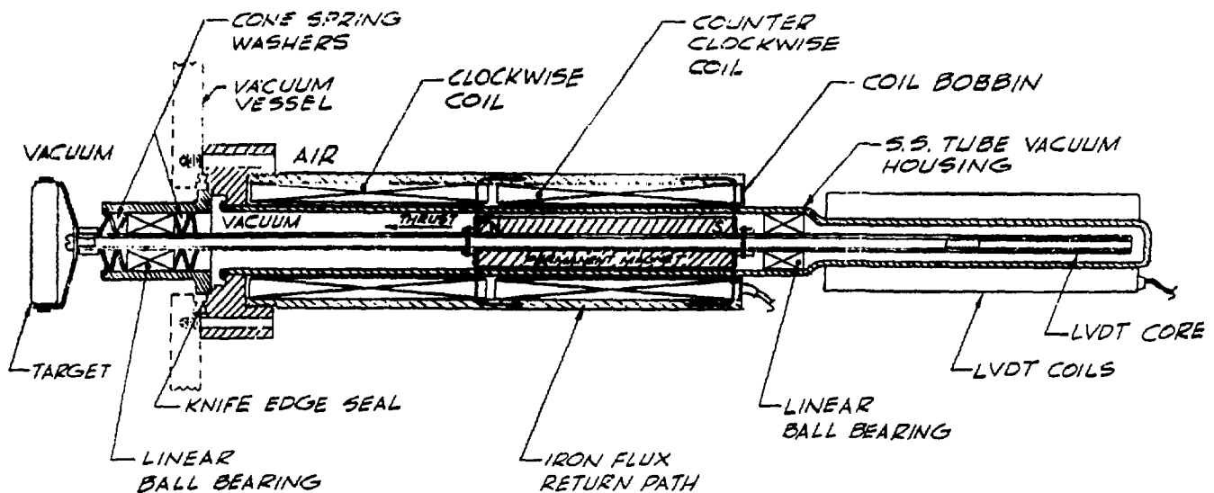
Figure 1. Beam scraper assembly (not to scale).
