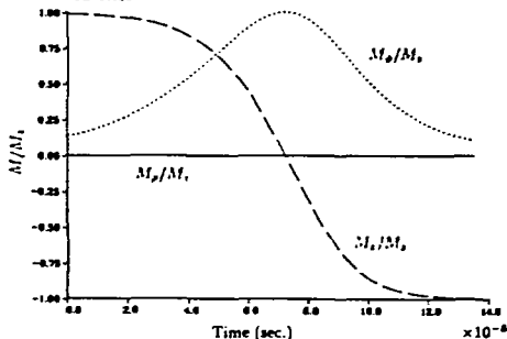
Fig. 3. Components of \vec{M}(t) at radial position \rho = a/2 . M_x , while small compared with M_s , produces a radial demagnetizing field that becomes comparable to the applied field.
