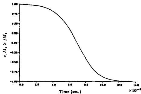
Fig. 2. \langle M_x(t) \rangle averaged over all radii for \epsilon_r = 12 , M_s = 300 KA/m, B_0 = 9.42 \times 10^{-4} T, k_d = 4 , \gamma = -275 rad-sec ^{-1} \cdot T^{-1} , and a = 10 cm, which values are chosen to be representative of the ATA linac cavities.
