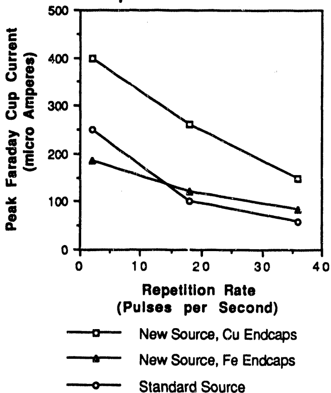
Fig. 3. Performance of various source models versus repetition rate. Intensity is measured at the entrance to the SuperHILAC Alvarez linac. The three curves represent two new versions, one with copper endcaps and the other with iron endcaps, both with a 19 mm long slit, and one older version with an 11 mm long slit.
