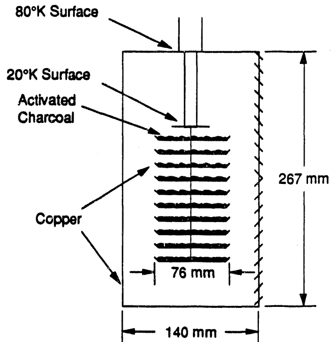
Fig. 4. Cryogenic pumping array, composed of copper with activated charcoal adsorbent.
