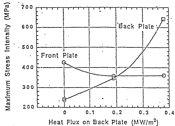
Figure 3 Variations of the maximum stress intensity in the front and back plates of the first wall as a function of the heat flux on the back plate for a 4 \times 4 \times 5 \text{ mm} first wall design.
