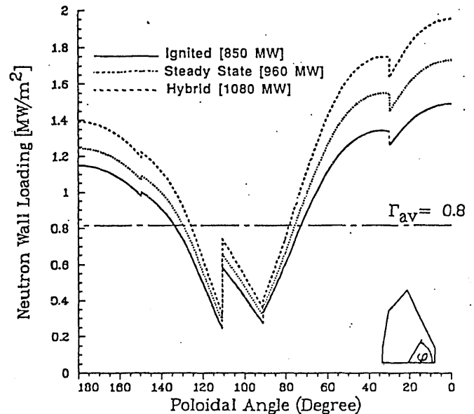
Figure 2 HARD neutral wall loading for the three modes of operation.
