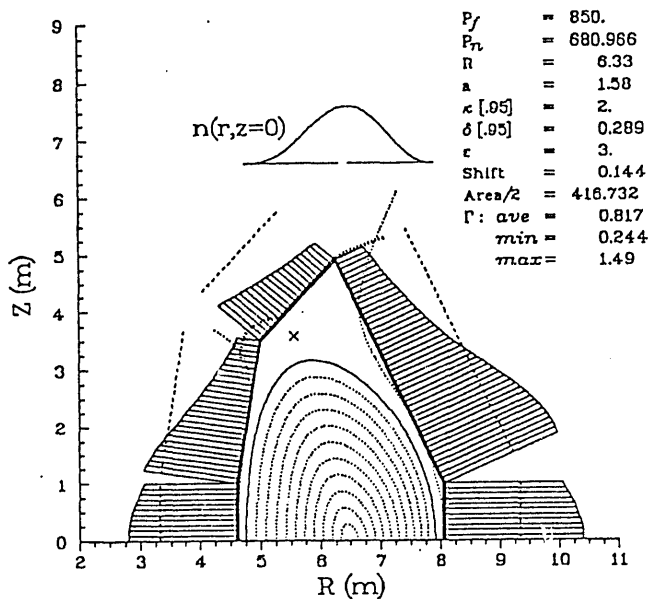
Figure 1 HARD first wall model and neutron wall loading for the ignited mode.
