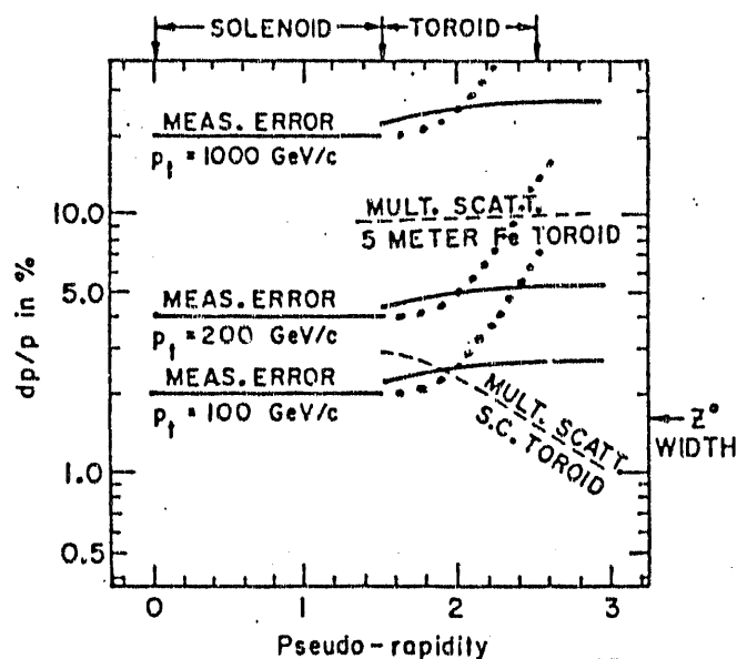
Fig. 1. Comparison of the muon momentum resolution of the SDC superconducting air-core toroid system with that of the central tracker. The solid lines show the resolutions dp_T/p_T^2 = 0.2 (TeV/c) -1 for the central tracker and 0.25 (TeV/c) -1 \cos\theta for the air-core toroids. The dashed lines show multiple-scattering contributions to the resolution of an air-core toroid and a toroid of magnetized iron. The dotted lines show the resolution which might be chosen for a small angle silicon strip tracking system in the solenoid region. Also shown is the resolution required to reconstruct the Z(+\mu\mu) mass with an error equal to the natural width of the Z .
