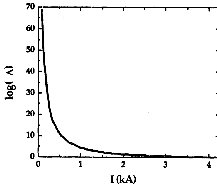
FIG. 3.10. The dimensionless mode area, \Lambda , of the HE_{11} mode of the ion-channel, decreases sharply as a function of beam current I for I \leq 2 kA. Plot of \log_{10}(\Lambda) versus I(\text{kA}) shows that \Lambda passes through about 70 orders of magnitude for I varying from 100 A to 4 kA.
