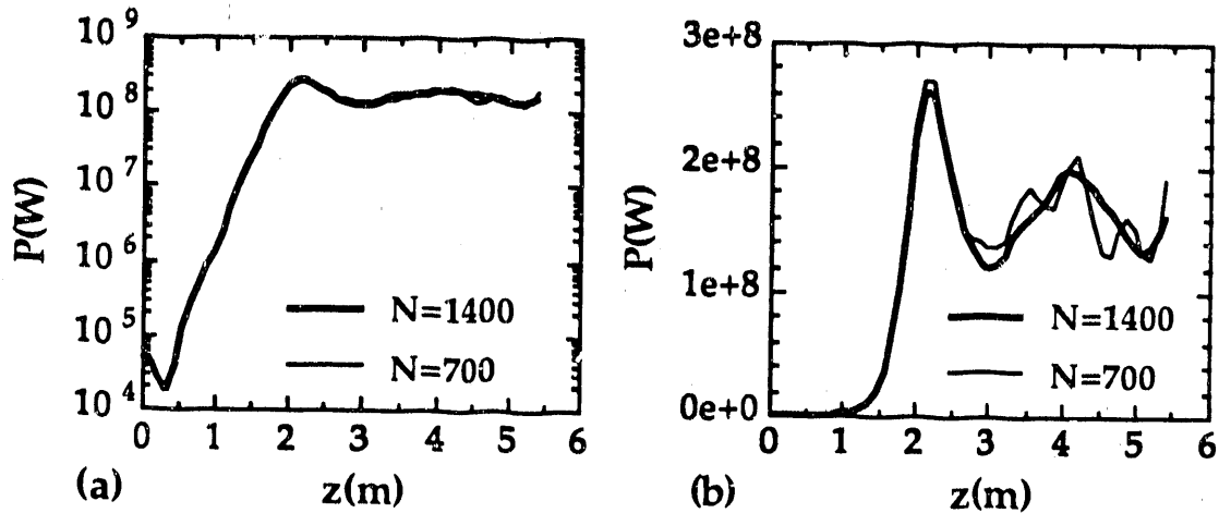
FIG. 4.21. Example of the insensitivity of the numerical result to a change in the number of particles used to model energy spread for N=700 and 1400, corresponding to 5 and 10 different h -values respectively and \sigma_h=35\% . In (a) we see that the linear growth rates agree well, and in (b) we see that the peak power levels agree well. Note that the larger number of particles has resulted in more realistic phase-mixing and a noticeably smoother power variation in (b).
