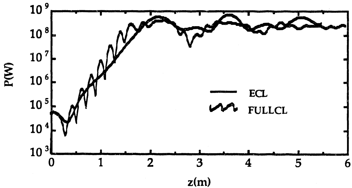
FIG. 4.15. The results from the code FULLCL (wiggling curve) and ECL, for power versus z , for the example of Table 4.1, including optical guiding. FULLCL predicts saturation at L_{sat} \sim 2.3 m, with P \sim 370 MW.
