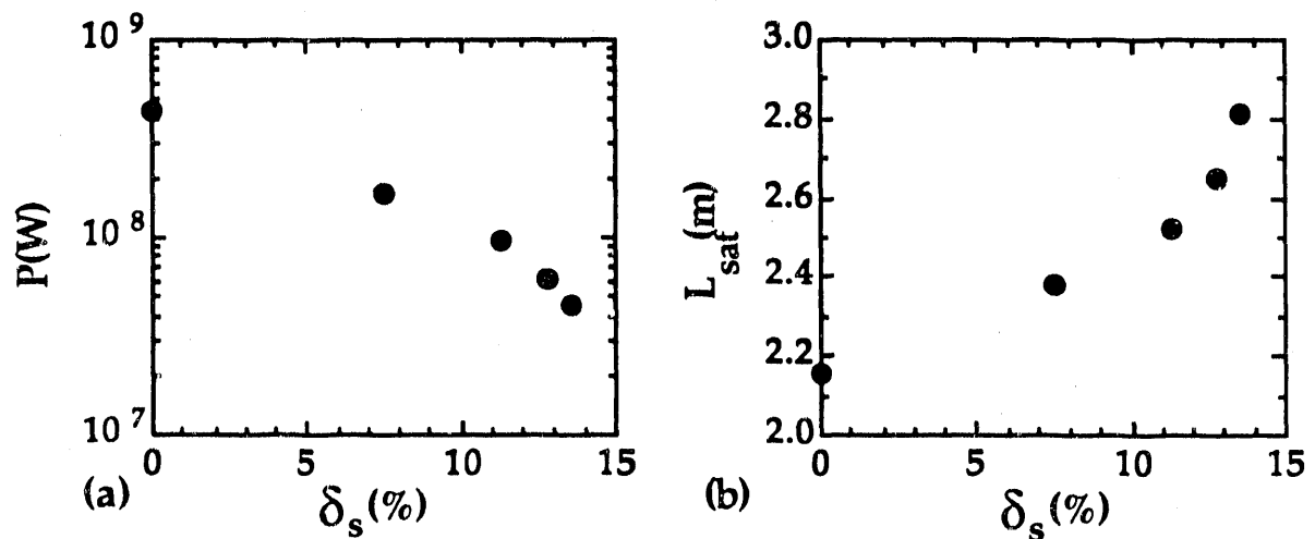
FIG. 4.18. (a) Power at saturation versus detuning spread, based on the data of Fig. 4.17, and (b) length for saturation. For these plots, the first appreciable peak in power was selected (even though, frequently, the second peak is the largest).
