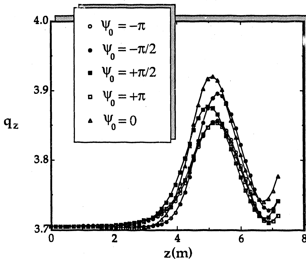
Fig. 4.10(b). Depicted is q_z versus z for the five representative low q_y particles of Fig. 4.9. Evidently, these particles gain energy near saturation ( z \sim 5 m).
