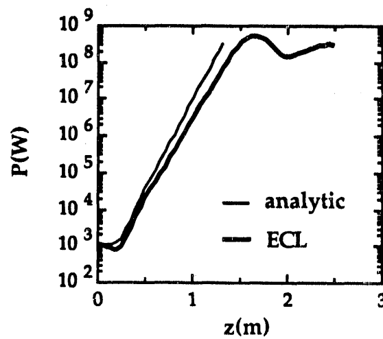
FIG. 4.24. Result for power vs z for the high gain example of Table 4.6, from ECL (dark curve) with a step-radial profile (no spread in transverse energy) compared to the analytic result (light curve).
