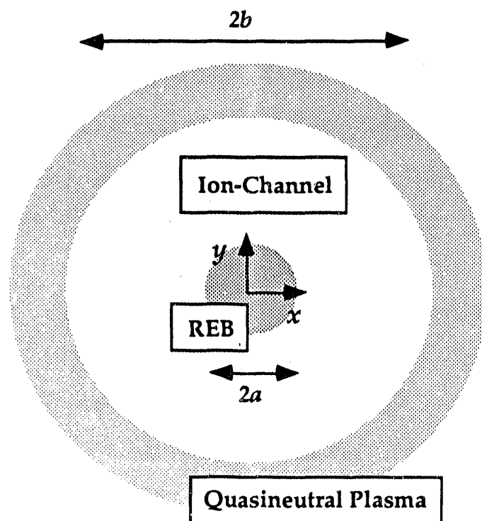
FIG. 2.8. An REB of radius a propagating through an underdense plasma, expels plasma electrons from the beam volume and beyond to produce an "ion-channel" of radius b \sim a(n_b/n_p)^{1/2} .
