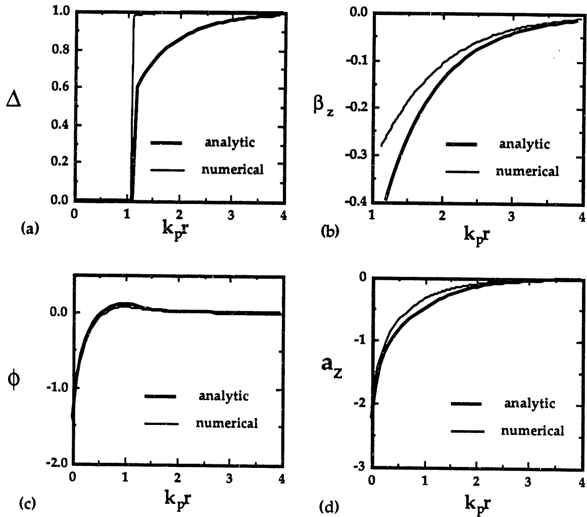
FIG. 2.5. Solution of Eq. (2.31) for \psi versus r , for U=1 ( I \sim 4 kA) compared to the analytic result of the V \ll 1 approximation. (a) \Delta = n_e/n_p , the plasma electron density normalized to its initial value (b) \beta_z = v_z/c , the plasma electron axial drift velocity (c) the scalar potential and (d) the axial vector potential, normalized by e/mc^2 . Evidently at V \sim 1 , the small V approximation is fair for the potentials, while it errs noticeably for the plasma electron density.
