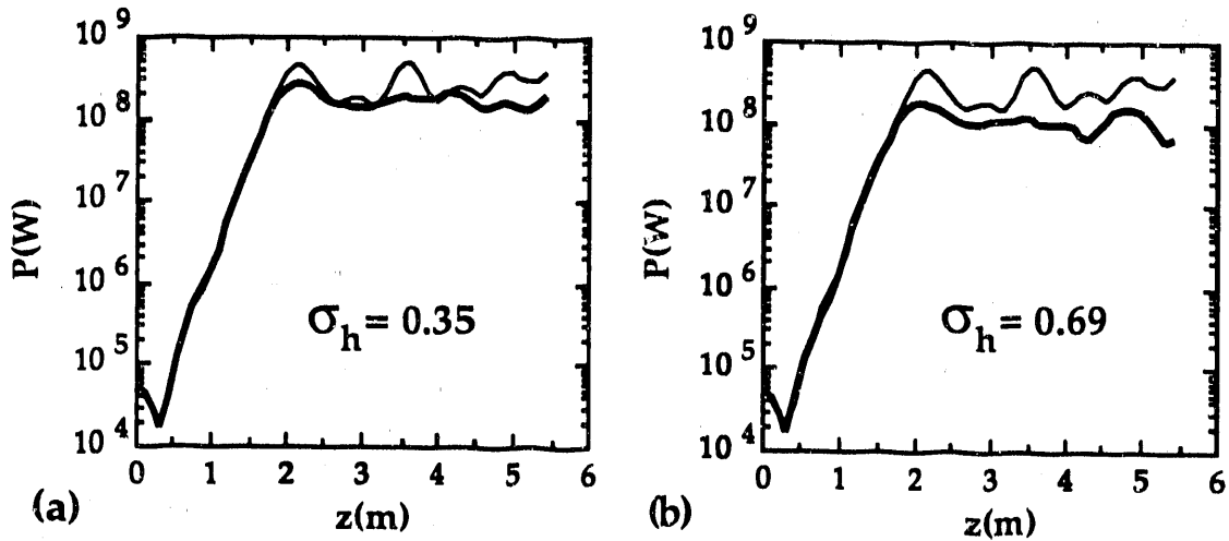
FIG. 4.20. ECL results for power versus z with fractional rms spreads in transverse energy (dark curves) of (a) 35% and (b) 70% (dark curves), compared to the cold beam result of Fig. 4.14 (light curve). (a) For the parabolic beam of the peak power is 270 MW, at 2.2 m, (56% of the step-profile result). (b) For the case of \sigma_h comparable to a Gaussian beam, the peak power is 173 MW at 2.1 m (36% of the step-profile result).
