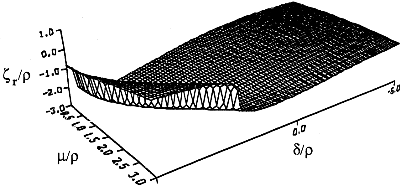
FIG. 3.6. (b) The real part of the root \zeta_r = \text{Re}(\zeta_{\pm}) is plotted versus detuning, \delta and the cold beam dielectric parameter \mu , as in Fig. 3.6(a). Note that \text{Re}(\zeta) = -(\Gamma_i + \Delta\omega)/\omega_p < 0 in regions where \text{Im}(\zeta) \propto \text{Re}(\Gamma) > 0 (i.e., in regions where amplification occurs) as would be expected from the discussion of the ponderomotive force of Eq. (3.70).
