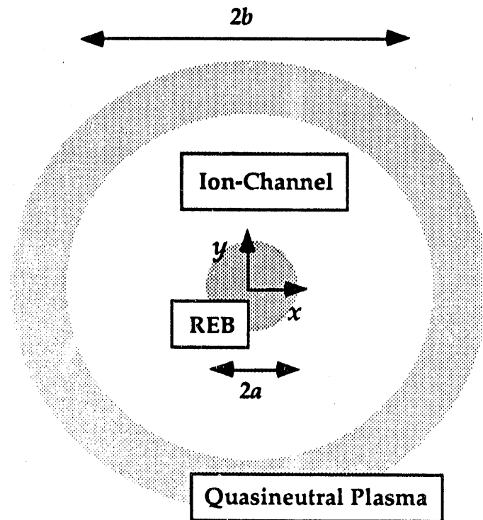
FIG. 3.1. (a) An REB, propagating through an underdense plasma, expels plasma electrons from the beam volume and beyond to produce an "ion-channel", which then focusses the beam, and causes it to radiate.
