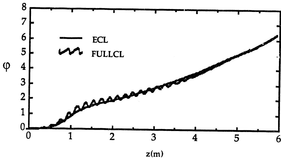
FIG. 4.5. Comparison of the phase advance computed by the ECL code (smooth curve) with that of FULLCL (tortuous curve).
