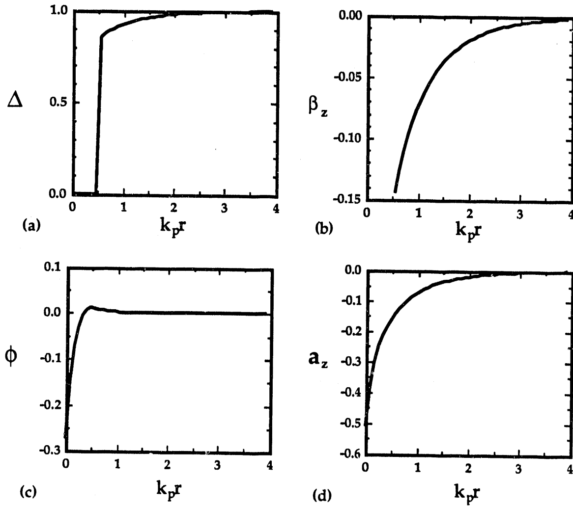
FIG. 2.4. The analytic solution in the large skin-depth approximation for U=0.5 ( I \sim 1 kA). (a) \Delta = n_e/n_p , the plasma electron density normalized to its initial value (b) \beta_z = v_z/c , the plasma electron axial drift velocity (c) the scalar potential and (d) the axial vector potential, normalized by e/mc^2 . Due to the axial drift depicted in (b), electrons are "held off" the channel wall by the v \times B force and this is reflected in the droop in the density in (a). This deficit of charge at the wall produces a small potential trough as depicted in (c), just adequate to balance the v \times B force for the remaining electrons.
