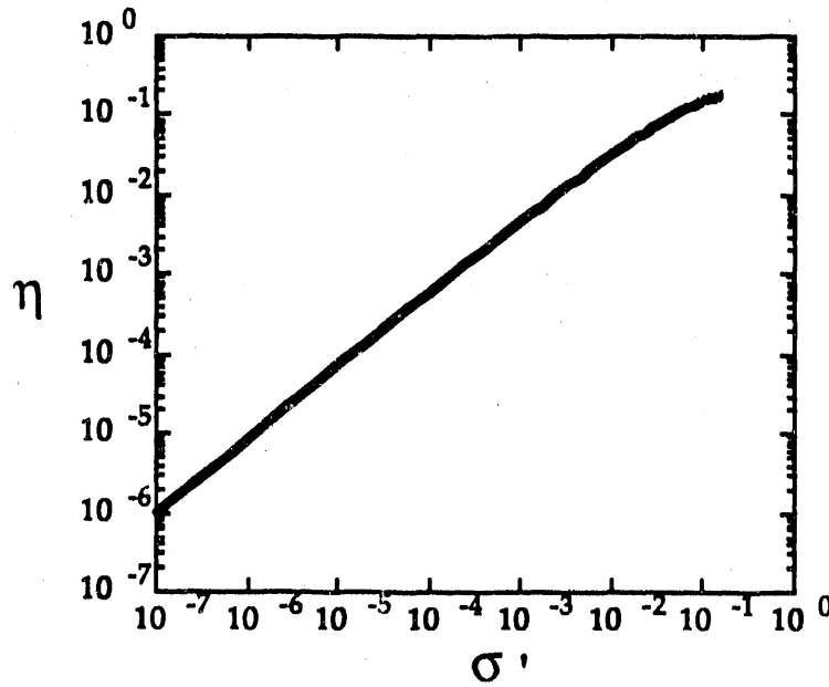
FIG. 3.15 (b) The overlap integral for the optically guided mode in the limit of large detuning, as a function of the dimensionless parameter \sigma' = 8a\beta^2 |\delta| , corresponding to the solution of Eq. (3.258) as depicted in Fig. 3.15(b). For \sigma' < 10^{-3} , this result is well-fit by \eta \sim 2.032 (\sigma')^{0.903} .
