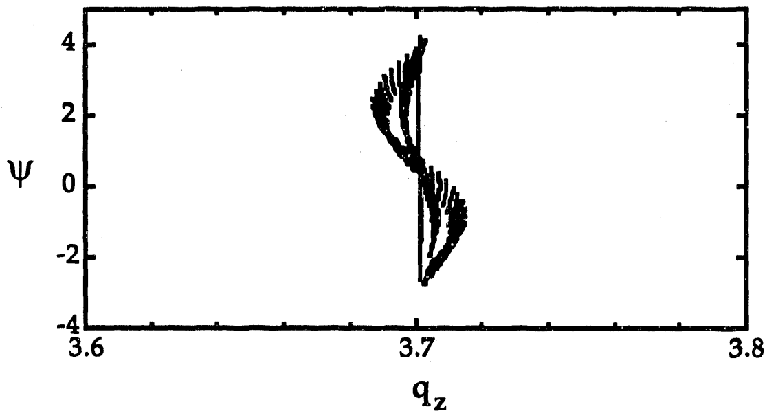
Fig.4.8 (b). Orbit segments for the particles of Fig. 4.8(a), for 0.7 < z < 1.1 m. We observe that some particles are remaining nearly stationary in q_z . These are just the particles initialized with small q_y .
