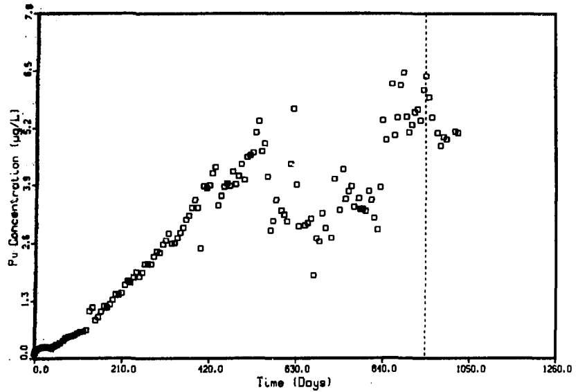
Fig. 7. Plutonium concentration versus time for aquarium number 23 (warm fresh water with a 33.5-g source). The vertical dashed line indicates removal of the source from the aquarium.
