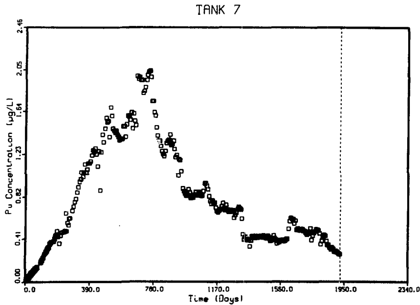
Fig. 6. Plutonium concentration versus time for aquarium number 7 (cold sea water with a 6.1-g source). The vertical dashed line indicates removal of the source from the aquarium.
