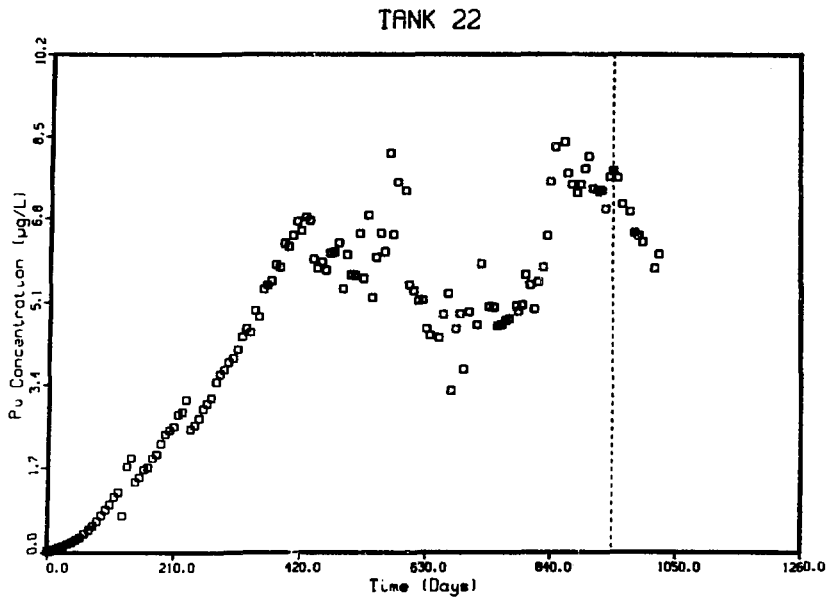
Fig. 5. Plutonium concentration versus time for aquarium number 22 (cold sea water with a 33.6-g source). The vertical dashed line indicates removal of the source from the aquarium.
