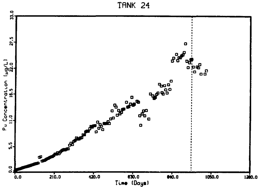
Fig. 2. Plutonium concentration versus time for aquarium number 24 (cold fresh water with a 33.6-g source). The vertical dashed line indicates removal of the source from the aquarium.
