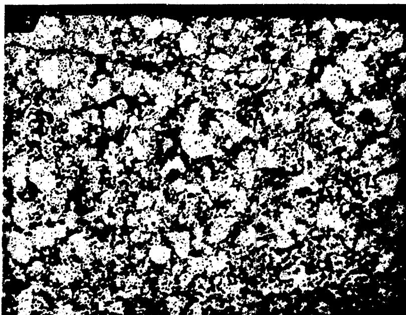
Fig. 12. A section of \text{PuO}_2 pellet number ET2-4 after etching. This source was exposed to fresh water at 35^\circ\text{C} for 943 days. Examination of the edge of the source, at the top of the photomicrograph, reveals no evidence of attack by the etching solution. The magnification is 100X.
