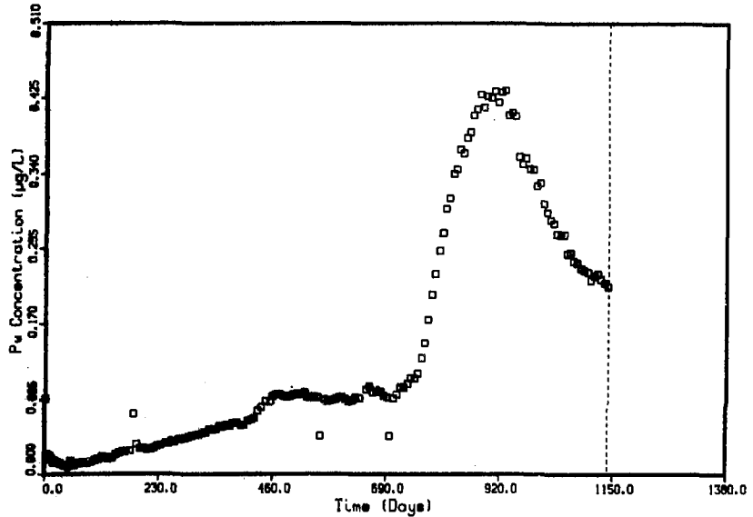
Fig. 8. Plutonium concentration versus time for aquarium number 12 (warm sea water with a 63.2-g source). The vertical dashed line indicates removal of the source from the aquarium.
