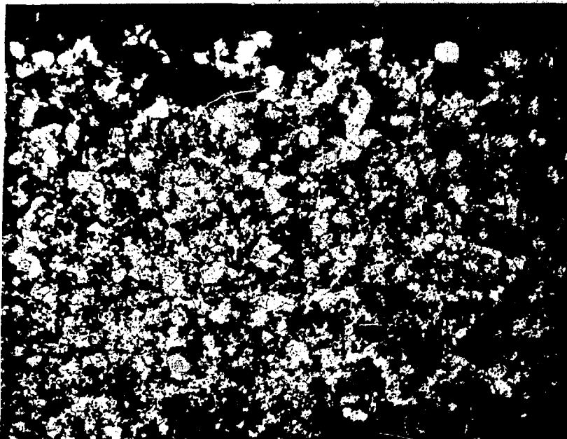
Fig. 11. A section of \text{PuO}_2 pellet number ET2-6 after etching. This source was exposed to simulated sea water at 35^\circ\text{C} for 943 days. The effects of the etching treatment are clearly visible at the top edge of the photomicrograph. The magnification is 50X.
