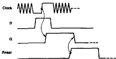
Figure 2. Timing Diagram at MC10H131P flip-flop.
