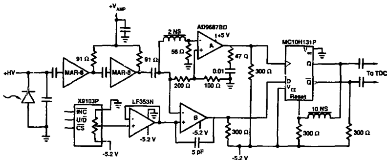
Figure 1. Time-of-flight circuit.
