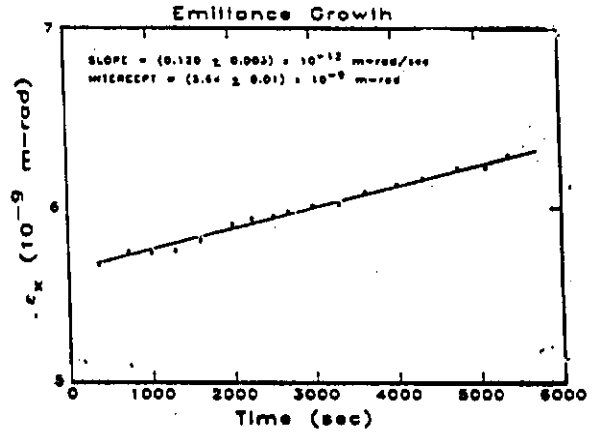
Fig. 1. Horizontal emittance as a function of time in the Tevatron.
