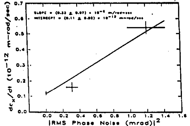
Fig. 2. Fit of horizontal emittance as a function of phase noise amplitude in 100 Hz binwidth.
