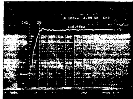
Figure 7a - Proton
