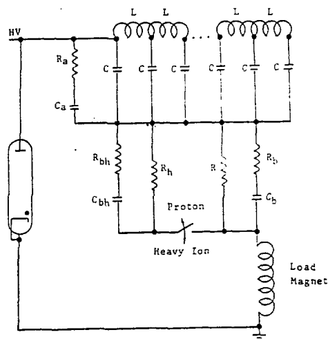
Figure 1 - Circuit Diagram of Test Pulser
