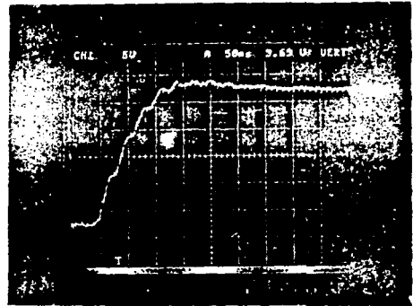
Figure 6a - Proton
