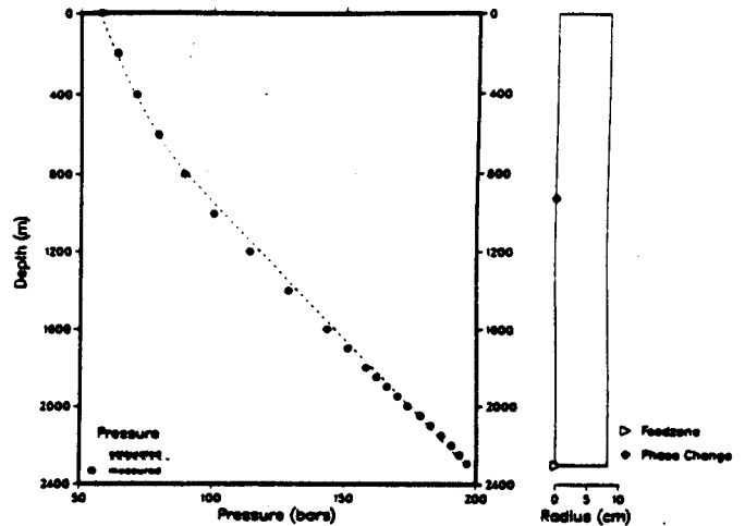
CERRO PRIETO, Well M-91 Wellbore calculations during discharge Measurements from FEB-8-1978
