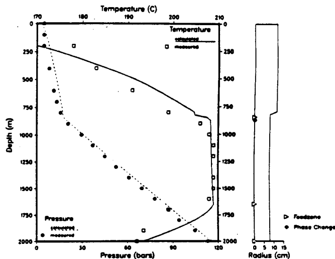
Olkaria, well OW-201 Wellbore calculations during discharge Measurements from 22-oct-1984
