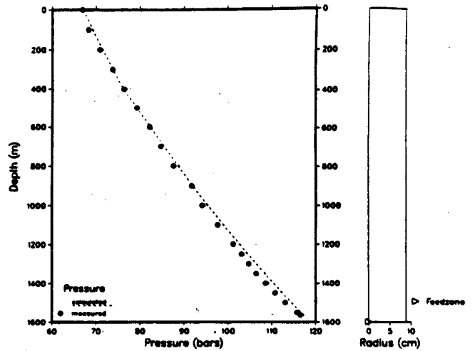
CERRO PRIETO, Well M-51 Wellbore calculations during discharge Measurements from Feb-20-1978
