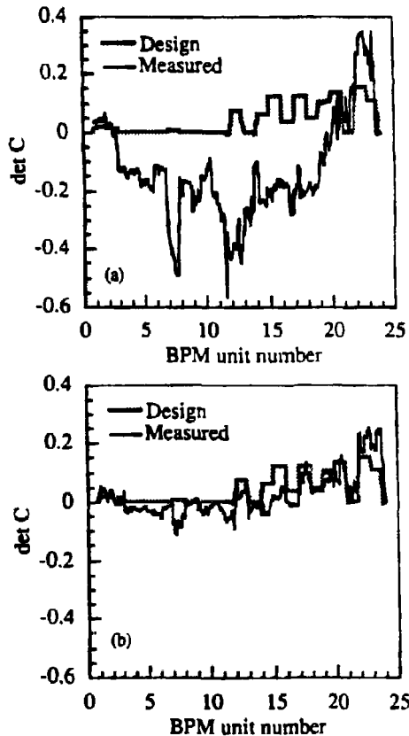
Fig. 3 North Arc det C (a) after PHASEFIX and (b) after application of vertical and horizontal 3\pi bumps.
