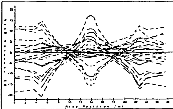
Figure 2: Particle Orbit with a 0.1 mm rms Quadrupole Misalignment
