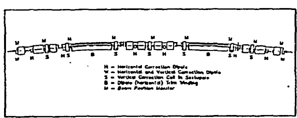
Figure 1: APS Storage Ring Cell Without Straight Sections
