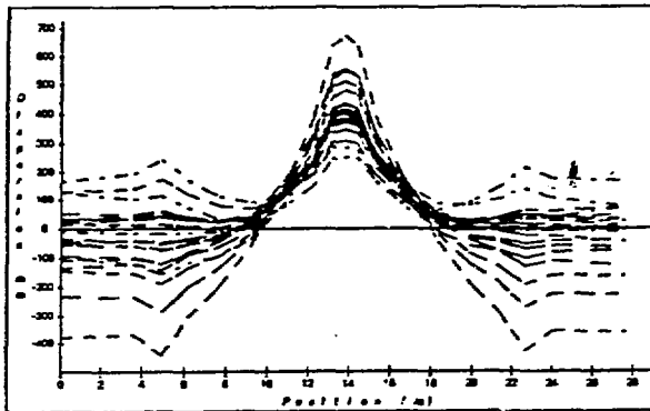
Figure 3: Horizontal Dispersion with a 0.1 mm rms Quadrupole Misalignment
