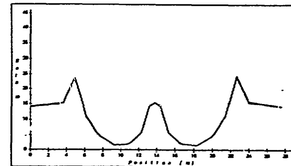
Figure 7: Horizontal Beta after Correction of a 0.1 mm rms Quadrupole Misalignment
