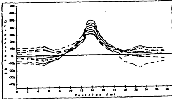
Figure 9: Horizontal Dispersion Function with a Gradient Field Error of 1% in the Quadrupole Magnets
