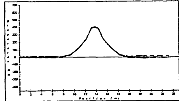
Figure 6: Horizontal Dispersion after Correction of a 0.1 mm rms Quadrupole Misalignment
