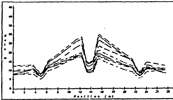
Figure 10: Vertical Beta Function with a Gradient Field Error of 1% in the Quadrupole Magnets
