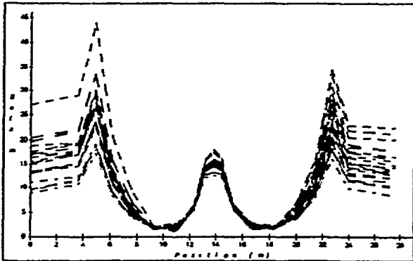
Figure 4: Horizontal Beta Functions with a 0.1 mm rms Quadrupole Misalignment
