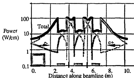
Figure 2. Distribution of radiation in the antechamber.
