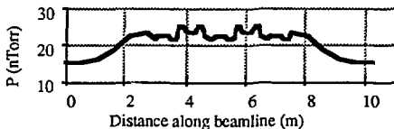
Figure 5. Pressure in the antechamber.
