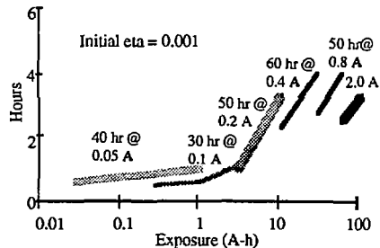
Figure 6. Beam lifetime during commissioning.
