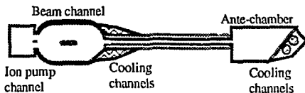
Figure 3. Ante-chamber cross section for the phi factory.
