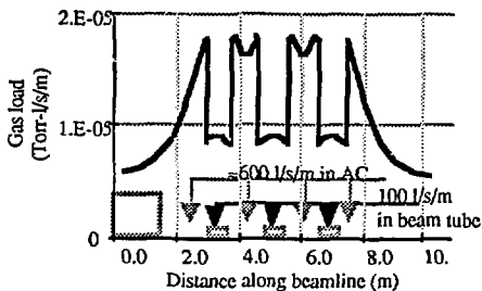
Figure 4. Distribution of gas load and pumping in SMC.
