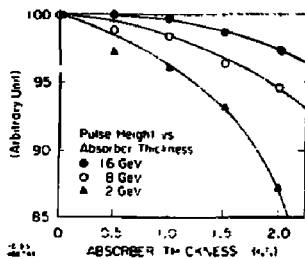
Fig. 6. Relative pulse height versus absorber thickness for energies of 2 GeV, 8 GeV and 16 GeV.
