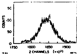
Fig. 2. Pulse height spectrum of positrons with energy of 17.5 GeV for a 20X_0 lead glass counter. The solid curve is a Gaussian fit to the data.
