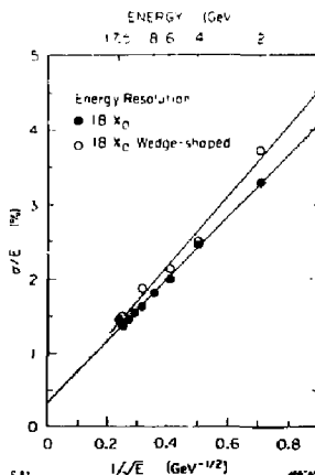
Fig. 9. Energy resolution for a wedge-shaped lead glass block of 18X_0 (open circles). Energy resolution for the normal block of 18X_0 is shown for comparison (closed circles).
