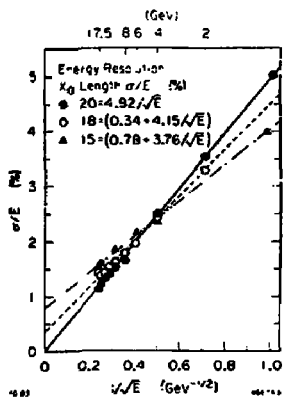
Fig. 3. Energy resolution for 15X_0 , 18X_0 , and 20X_0 blocks.
