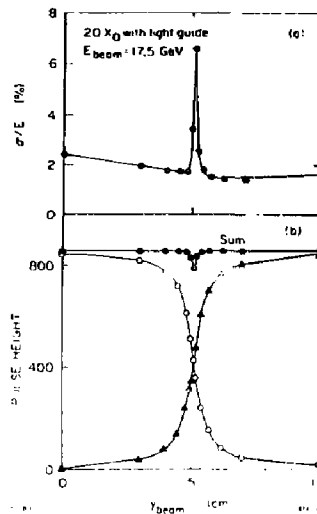
Fig. 8 Beam position dependence of the pulse height for a 20X_0 lead glass block with light guide for a beam energy of 17.5 GeV.
