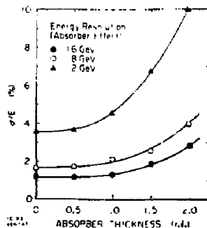
Fig. 5. Energy resolution versus absorber thickness for energies of 2 GeV, 8 GeV and 16 GeV.
