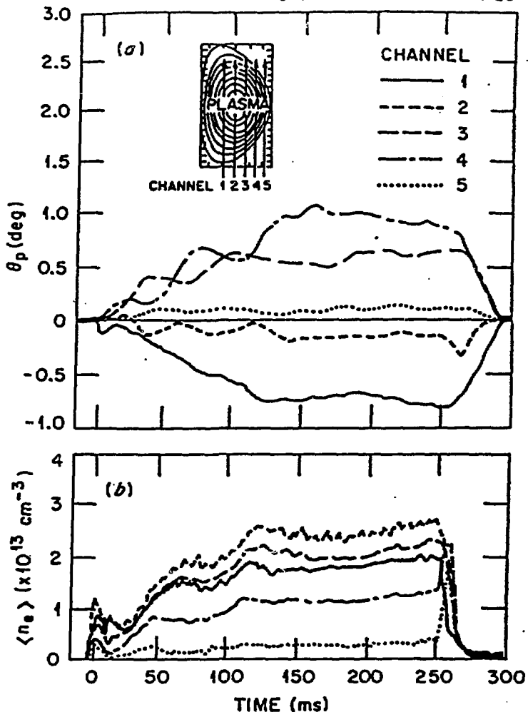
Fig. 1. Time variation of (a) Faraday rotation and (b) line-averaged electron density measured by the multichord FIR interferometer/polarimeter system on ISX-B tokamak.
