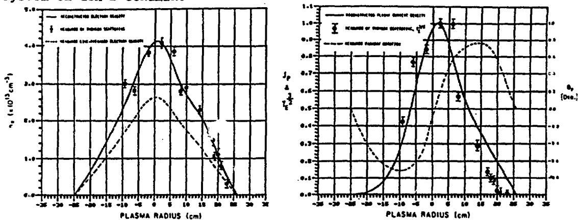
Fig. 2. Comparison of the reconstructed electron density and current density profiles with the profiles measured by Thomson scattering.
