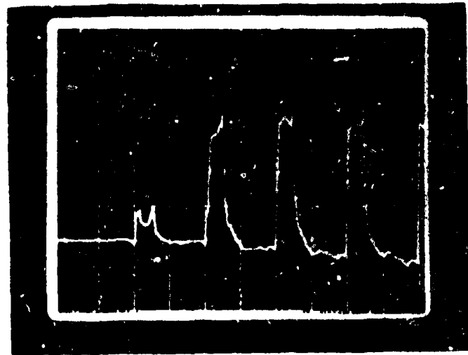
Fig. 2. Output beam current measured by B monitor; four of nine bunches are shown.
