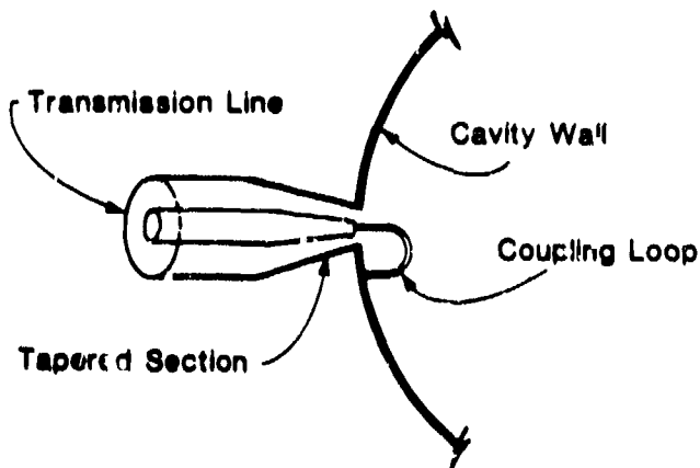
Fig. 4. Transmission line, loop, and cavity.
