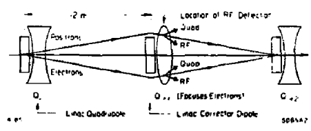
Fig. 2. A "magic" dipole bump corrects for static RF deflections given to electrons and positrons.
