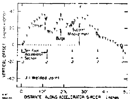
Fig. 6. Vertical survey of a girder, showing offsets, bulges, and intragirder support misalignments before corrections.
