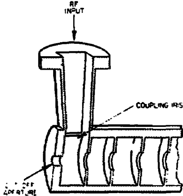
Fig. 3. SLAC disk-loaded accelerator showing a cross section of the cavities and end coupler.
