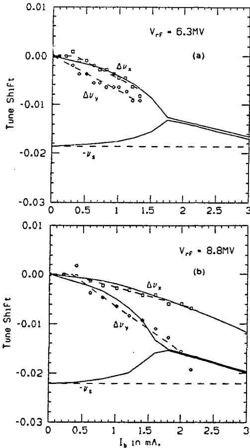
Fig. 2 Horizontal (squares) and vertical (diamonds) coherent tune shift as a function of bunch current for (a) the low-emittance lattice and (b) the modified low-emittance lattice. The dashed lines are the result of a linear fit to the measured data. The solid curves are the calculated tune shifts of the m = 0 and m = -1 modes calculated with BBI/MOSES.
