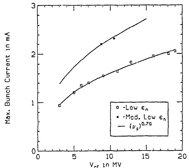
Fig. 1. The maximum single bunch current measured as a function of RF cavity voltage for the low-emittance tune (squares) and the modified low-emittance tune (dots). The curves are the result of a fit to a power law dependence on the synchrotron frequency of \nu_s^{0.79} .
