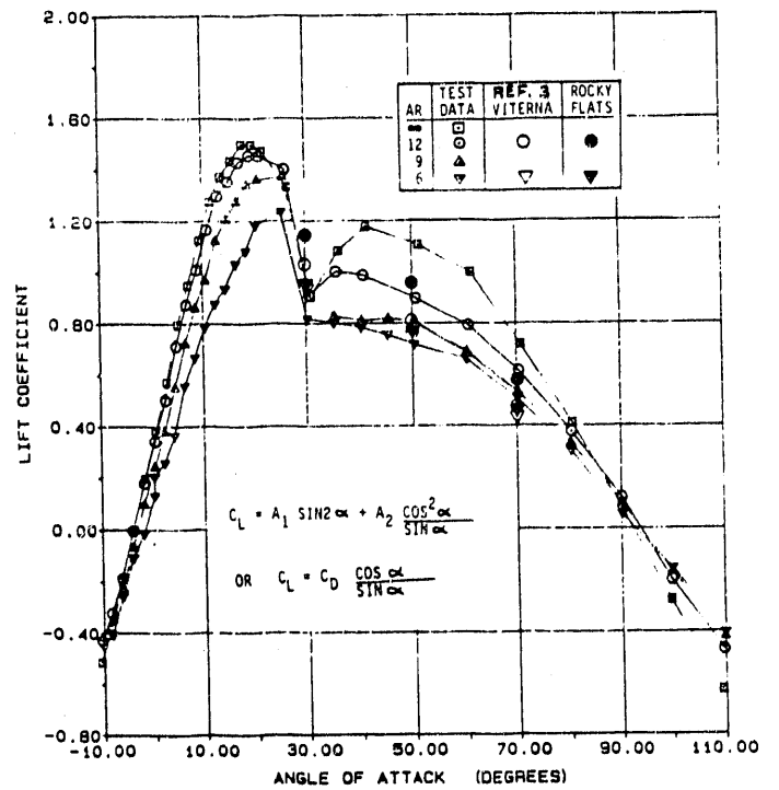
Fig. 2. Effect of Aspect Ratio on Lift Coefficients of the NACA 4418 Airfoil at Re = 0.25 \times 10^6 .
