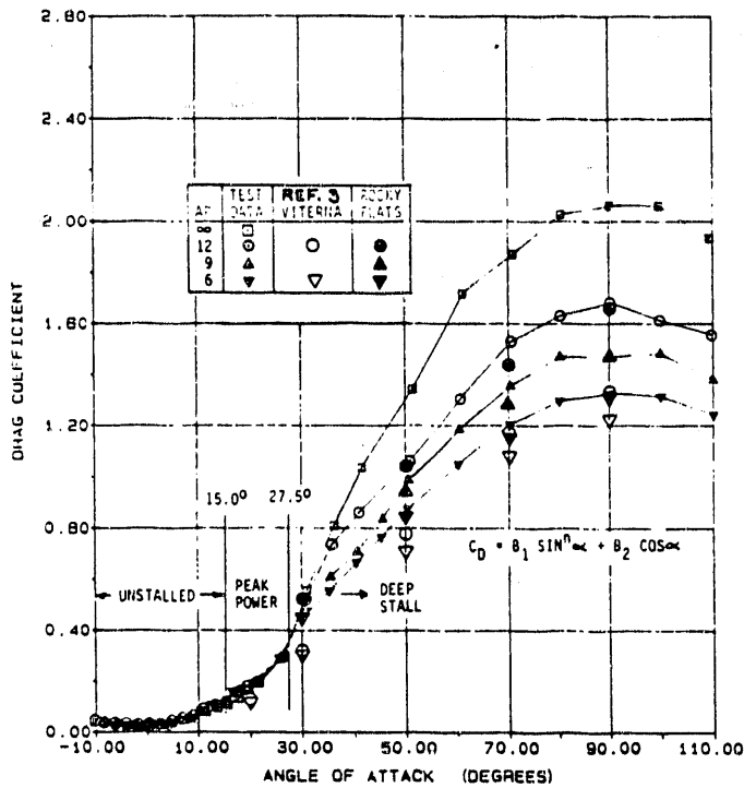
Fig. 1. Effect of Aspect Ratio on Drag Coefficients of the NACA 4418 Airfoil at Re = 0.25 \times 10^6 .
