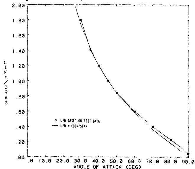
Fig. 3 Effect of Aspect Ratio on Lift/Drage Ratio in Deep Stall
