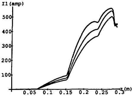
Figure 3 RF current as a function of z ( E=440 kV)
