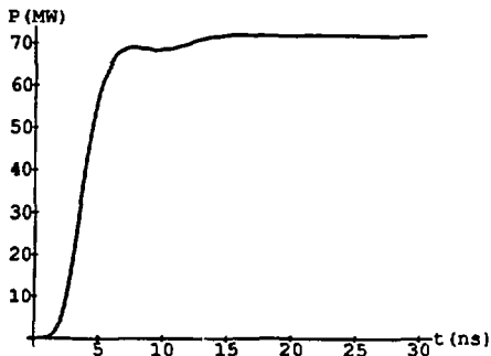
Figure 2 Output power as a function of time (E=440 kV)
