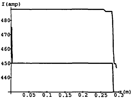
Figure 4 DC current as a function of z
