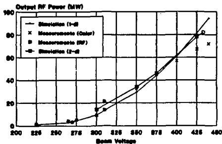
Figure 1 Output power as a function of beam energy: simulation and experiment
