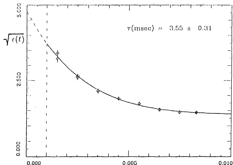
Figure 2. Linac wire scanners: extracted beam emittance vs. time (sec)
