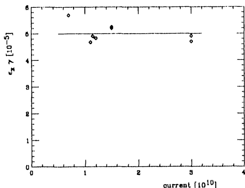
Fig. 5 emittance in sector 2 vs. current
