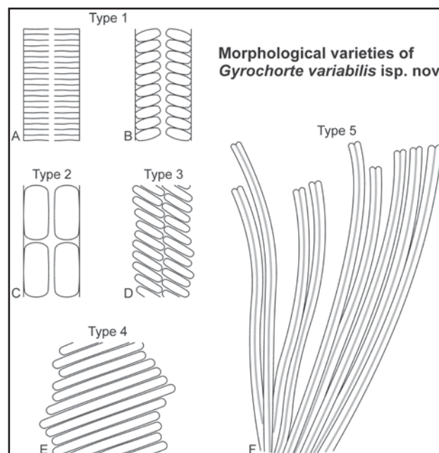
Figure 11: Sketch of the different morphological bedding-plane expressions of Gyrochorte variabilis isp. nov. Type 1: predominantly transverse ridges and biserially arranged pads. Type 2: biserially arranged pads, elongated in the direction of the ribbon and oblique with respect to the horizontal plane. Type 3: biserially arranged elongated pads, long axis of pads forming an angle with the direction of the ribbon. Type 4: Elongated pads forming an oblique angle with the direction of the ribbon (Fig. 7C). A biserial arrangement is no longer visible. Type 5: fan-like arrangement of bilobate rays. Types 3 to 5 are stages of a morphological continuum.
