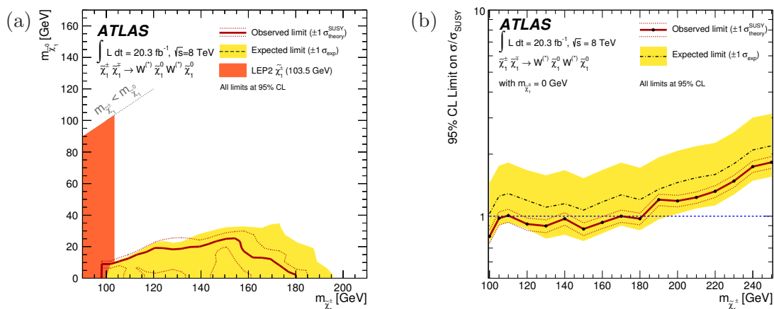
Figure 6. (a) Observed and expected 95% CL exclusion regions in the (m_{\tilde{\chi}_1^\pm}, m_{\tilde{\chi}_1^0}) plane for simplified-model \tilde{\chi}_1^\pm \tilde{\chi}_1^0 production followed by W -mediated decays. Also shown is the LEP limit [36, 37] on the mass of the chargino. (b) Observed and expected 95% CL upper limits on the cross-section normalized by the simplified-model prediction as a function of m_{\tilde{\chi}_1^\pm} for m_{\tilde{\chi}_1^0} = 0 .
