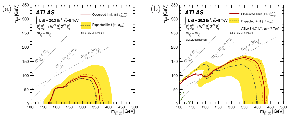
Figure 7. (a) Observed and expected 95% CL exclusion regions in the (m_{\tilde{\chi}_2^0}, m_{\tilde{\chi}_1^0}) plane for simplified-model \tilde{\chi}_1^\pm \tilde{\chi}_2^0 production followed by W and Z -mediated decays obtained from SR- Z jets; and (b) the exclusion regions obtained by combining with the ATLAS three-lepton search [83]. The green lines in (b) indicate the regions excluded by ATLAS using 4.7 \text{ fb}^{-1} of \sqrt{s} = 7 \text{ TeV} data [105].
