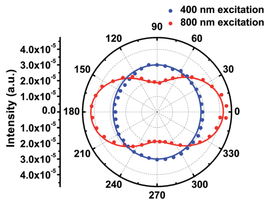
Fig. 4 Polar plot of the integral fluorescence intensity of the hybrid Ag nanowire–CdTe QD structure as a function of \theta (defined in Fig. 2b) under excitation of (a) 800 nm at 600 \mu\text{W} and (b) 400 nm at 0.045 \mu\text{W} . The results are fitted with a cosine function (solid lines).
