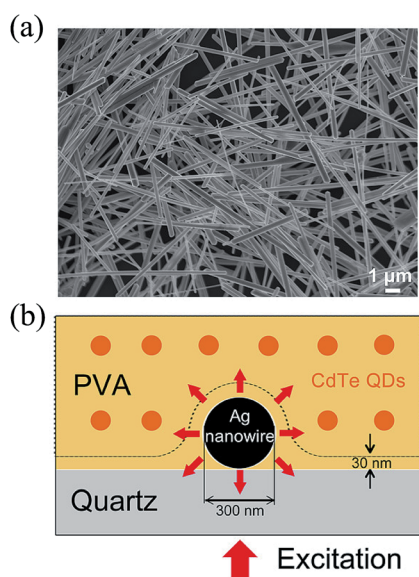
Fig. 1 (a) Scanning electron microscopy image of Ag nanowires. (b) Scheme of the plasmonic nanowire antenna functionalized by optical emitters (CdTe QDs) on top of a polyvinylalcohol (PVA) layer of 30 nm thickness. The surface plasmon of Ag nanowire antennas generated via the excitation of the incident laser pulse can near-field excite the CdTe QDs nearby with high efficiency to radiate the fluorescence.
