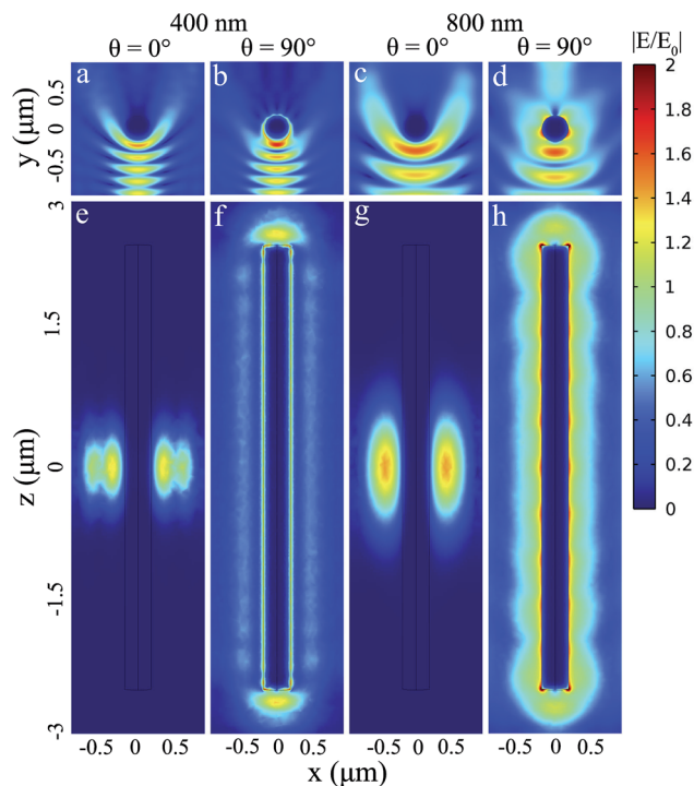
Fig. 6 Planar representations of the electric field E , around a Ag nanowire ( D = 300 nm, L = 5 \mu\text{m} ), relative to the incident field E_0 , |E|/|E_0| , simulated by the finite element method. The Ag nanowire is excited by a linearly polarized Gaussian light beam with \lambda = 400 nm or 800 nm propagating in the y direction with the polarization parallel and perpendicular to the Ag nanowire axis respectively. The top panels are cross-sections of the nanowire in the x - y plane at z = 0 , the bottom panels are cross-sections of the x - z plane at y = 0 .
