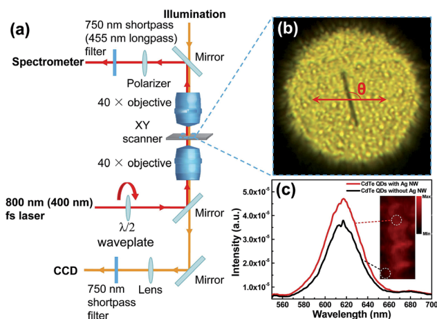
Fig. 2 (a) Scheme of the microscope photoluminescence measurement set-up. (b) Bright field image of the hybrid Ag nanowire–CdTe QD structure. \theta is the cross-angle between the Ag nanowire axis and the excitation laser polarization. (c) Two-photon excited fluorescence (TPEF) spectra with different excitation areas and fluorescence microscopy image of the hybrid structure, at the excitation power of 1 mW.
