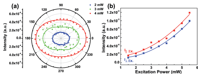
Fig. 3 (a) Polar plot of the TPEF intensity of the hybrid Ag nanowire–CdTe QD structure as a function of \theta (defined in Fig. 2b) under excitation at 800 nm, with the excitation power of 2 mW (blue dots), 3 mW (green dots), and 4 mW (red dots). The data exhibit a cosine angular dependence (solid lines). (b) The TPEF intensity at parallel ( I_{\parallel \text{Ex}} ) (red squares) and perpendicular ( I_{\perp \text{Ex}} ) (blue squares) polarized excitation fitted with a quadratic functional form (solid lines) as a function of the excitation power.
