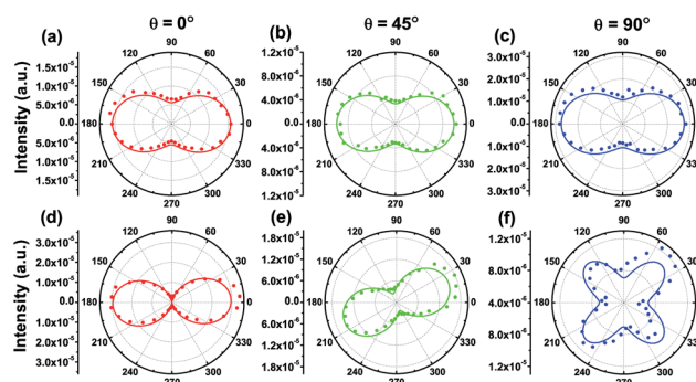
Fig. 5 The fluorescence intensity as a function of the angle between the Ag nanowire axis and the detected polarization direction, with \theta (defined in Fig. 2b) = 0^\circ , 45^\circ , and 90^\circ , under the excitation of (a–c) 400 nm and (d–f) 800 nm. The results are fitted with a cosine function (solid lines).
