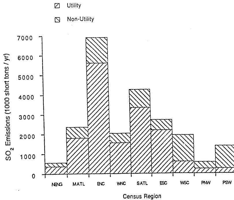
Figure 2. Distribution of SO 2 by Region From Utilities and Other Sources
