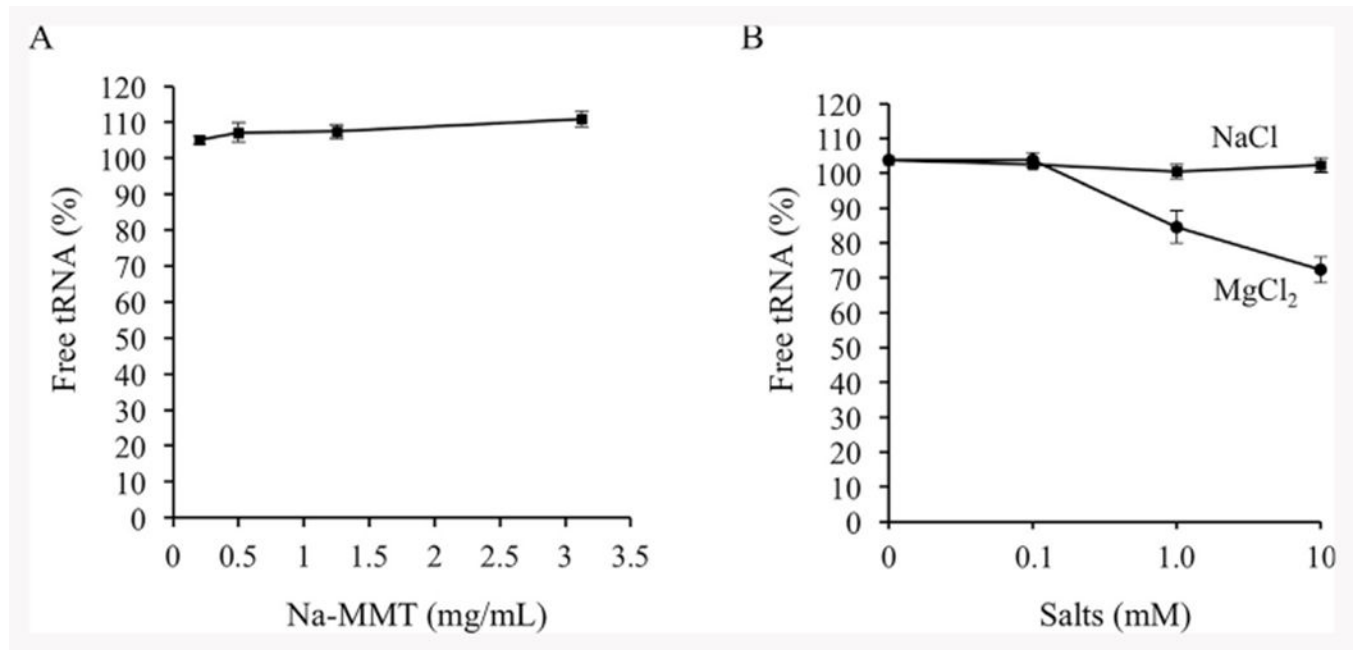
Fig. 4. Adsorption of complex tRNA molecules to Na-MMT. (A) Percentage of RNA remaining free when increasing amounts of clay are added to the binding reactions. (B) Assessment of binding to 0.5 mg/mL clay with and without addition of 10 mM NaCl or MgCl 2 .
