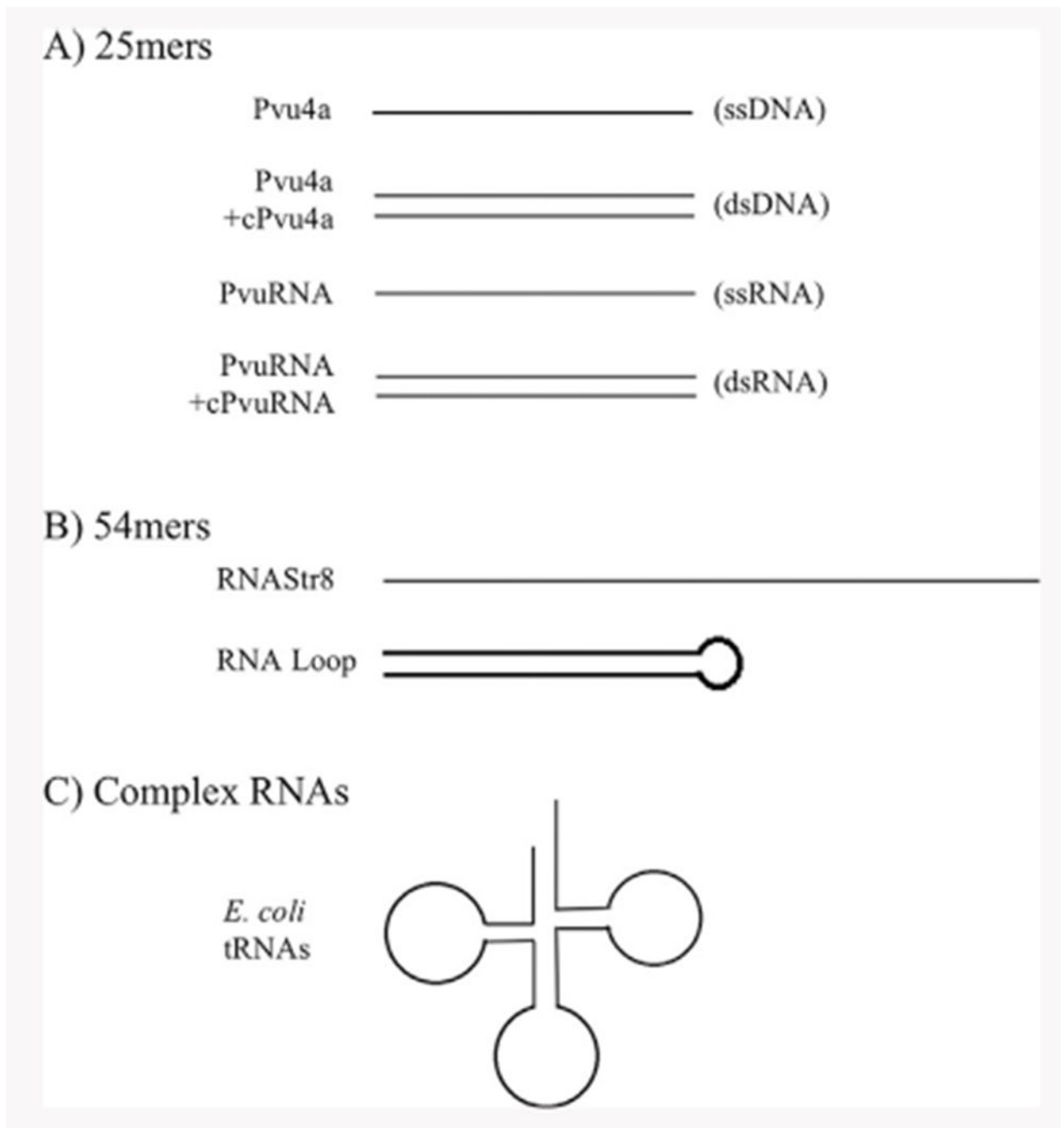
Fig. 1. Schematic representations of the different types of nucleic acids used in the study. (A) Oligonucleotide 25mer names are listed on the left side and single-stranded (ss) or double-stranded (ds) structure is indicated on the right side. Double-stranded 25mers were prepared by annealing complementary single-stranded 25mers and confirming by gel electrophoresis. (B and C) Structural representations of 54mers and 75–80 nt transfer RNAs. The 54mer RNAstr8 cannot form stable secondary structures while the RNALoop 54mer naturally forms a 25 bp double-stranded stem region with a 4 nt ssRNA loop at one end.
