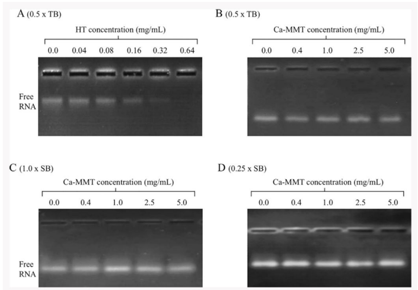
Fig. 7. Electrophoretic mobility shift assays can readily monitor formation of RNA:HT complexes but not RNA:Ca-MMT complexes. Assays were performed using 3.5% agarose gels and ssRNA 25mer PvuRNA. (A) Addition of increasing amounts of hydrotalcite (HT) to 200 ng ssRNA leads to disappearance of the free RNA band as HT:RNA complexes are formed. (B-D) In contrast to results with HT, MMT:RNA complex formation could not be monitored using conventional Tris-borate (TB) or other electrophoresis buffers such as sodium borate (SB).
