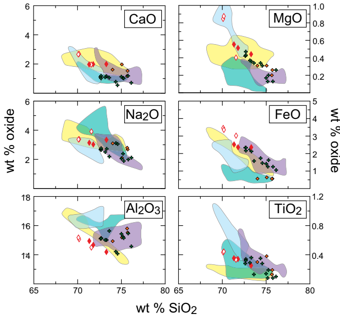
Figure 19. Silica versus major element oxides in Ash Mountain Complex (AMC) least evolved granites (LEGs) and experimentally produced melts (cf. Table 6) with SiO 2 contents >~68 wt%. Symbols and fields as in Figure 18.
