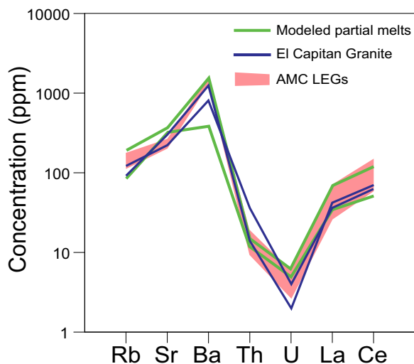
Figure 21. Calculated trace element abundances in partial melts produced in an experiment (run 1694) using Sierra Nevada batholith mafic source rock (green lines; see Fig. 6 and Table 5 in Ratajeski et al., 2005). Also shown are observed trace element abundances in two samples of the El Capitan Granite (blue lines) and Ash Mountain Complex (AMC) least evolved granites (LEGs) (pink shaded field).
