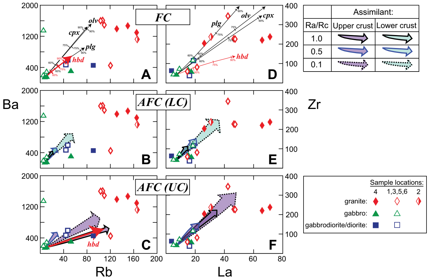
Figure 12. Trace element compositions of Ash Mountain Complex rocks and calculated trends for fractional crystallization (FC) and assimilation plus fractional crystallization (AFC) models. (A–C) Ba (ppm) versus Rb (ppm). (D–F) Zr (ppm) versus La (ppm). Symbols as in Figure 4. Mineral-melt distribution coefficients used in the models are given in Table 4. Arrows in A and D represent closed system Rayleigh FC processes involving olivine (olv), plagioclase (plg), clinopyroxene (cpx), or hornblende (hbd). Tick marks are shown for 60%, 75%, and 90% crystallization. In A, the hornblende fractionation trend is shown in red to distinguish it from the trend for plagioclase fractionation. Trends designated by arrows in B, C, E and F are for AFC processes, calculated using the equation given by DePaolo (1981). Except for C, each AFC trend encompasses individual vectors for removal of olivine, clinopyroxene, plagioclase, or amphibole to 90% crystallization (closed system equivalent). In C, the purple shaded arrows include individual vectors for removal of olivine, clinopyroxene or plagioclase, and the red arrows represents removal of hornblende; all trends represent to 90% crystallization (closed system equivalent). The narrow and broad red arrows represent rate of assimilation/rate of crystallization (Ra/Rc) 0.1 and from 0.5 to 1.0, respectively. See legend for the composition of the assimilant (either lower or upper crust [LC, UC]; from Rudnick and Fountain, 1995) and assumed Ra/Rc.
