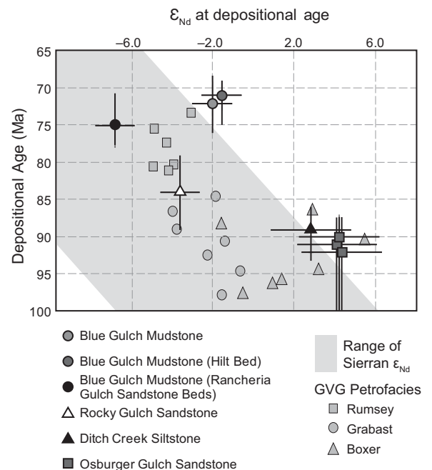
Figure 8. \epsilon_{\text{Nd}} versus depositional age for Hornbrook Formation and Great Valley Group (GVG) samples (GVG data from Linn et al., 1991). Range of Sierran \epsilon_{\text{Nd}} values is indicated in light-gray shading (values from DePaolo, 1981). Hornbrook Formation samples are shown with 1\sigma uncertainty.
